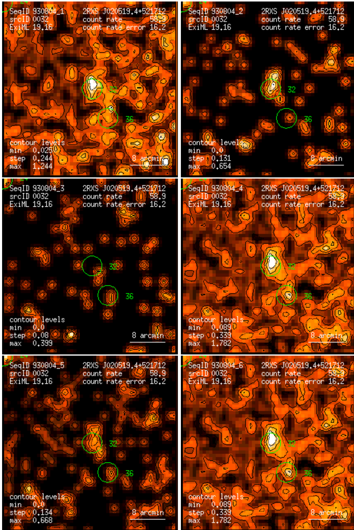
Figure 32: RASS 930804: detection 0032: band rate images, Gaussian filter: (1) PSPC channels 11 – 41, (2) 52 – 90, (3) 91 – 201, (4) 11 – 235, (5) 52 – 201, (6) 11 – 201. Broad band rates in counts/ks. Band rate contour levels in counts/ks/arcmin 2 .
