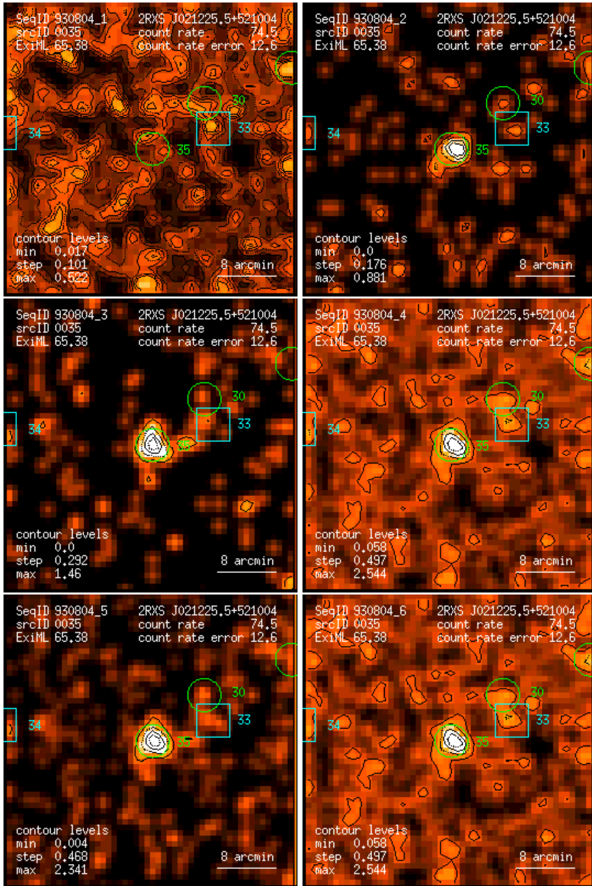
Figure 35: RASS 930804: detection 0035: band rate images, Gaussian filter: (1) PSPC channels 11 – 41, (2) 52 – 90, (3) 91 – 201, (4) 11 – 235, (5) 52 – 201, (6) 11 – 201. Broad band rates in counts/ks. Band rate contour levels in counts/ks/arcmin 2 .
