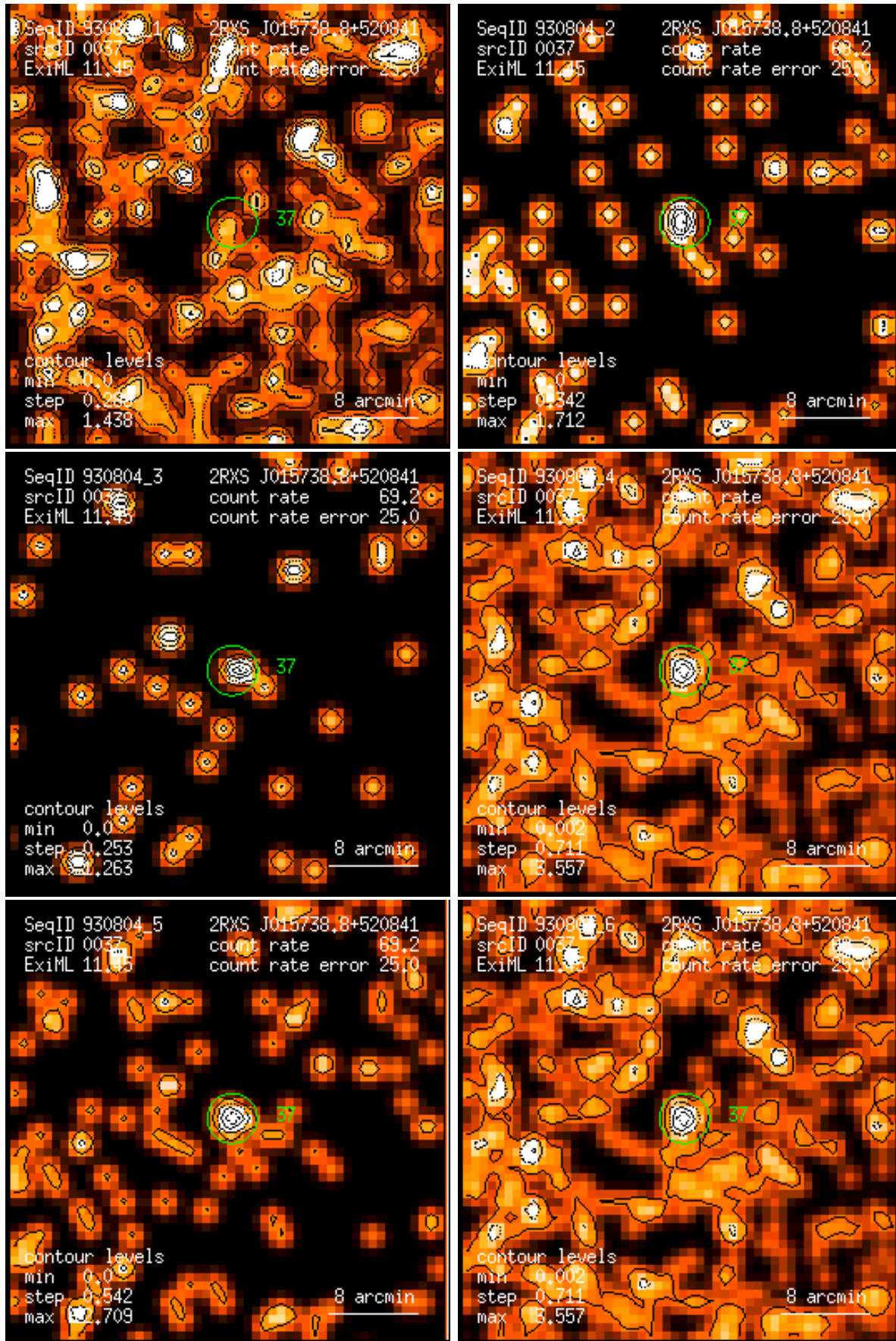
Figure 37: RASS 930804: detection 0037: band rate images, Gaussian filter: (1) PSPC channels 11 – 41, (2) 52 – 90, (3) 91 – 201, (4) 11 – 235, (5) 52 – 201, (6) 11 – 201. Broad band rates in counts/ks. Band rate contour levels in counts/ks/arcmin 2 .
