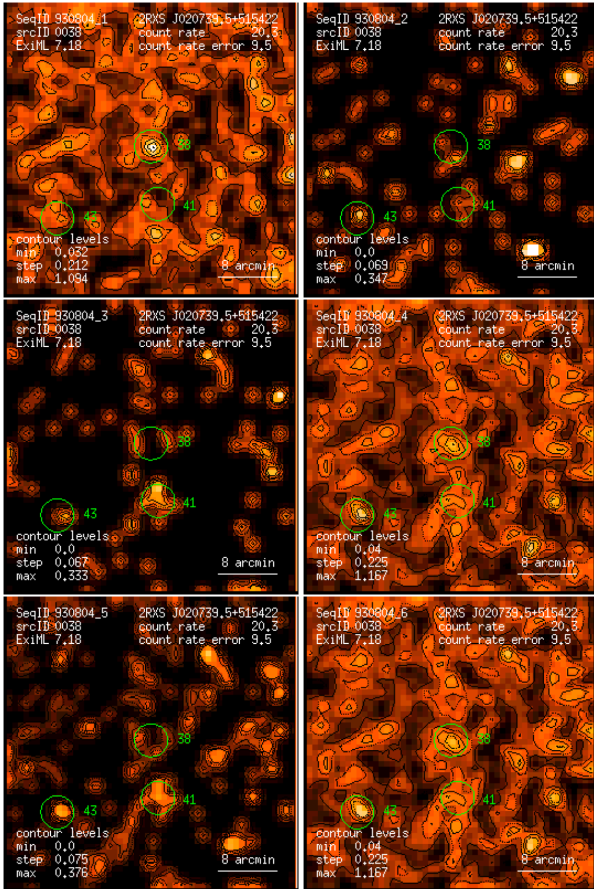
Figure 38: RASS 930804: detection 0038: band rate images, Gaussian filter: (1) PSPC channels 11 – 41, (2) 52 – 90, (3) 91 – 201, (4) 11 – 235, (5) 52 – 201, (6) 11 – 201. Broad band rates in counts/ks. Band rate contour levels in counts/ks/arcmin 2 .
