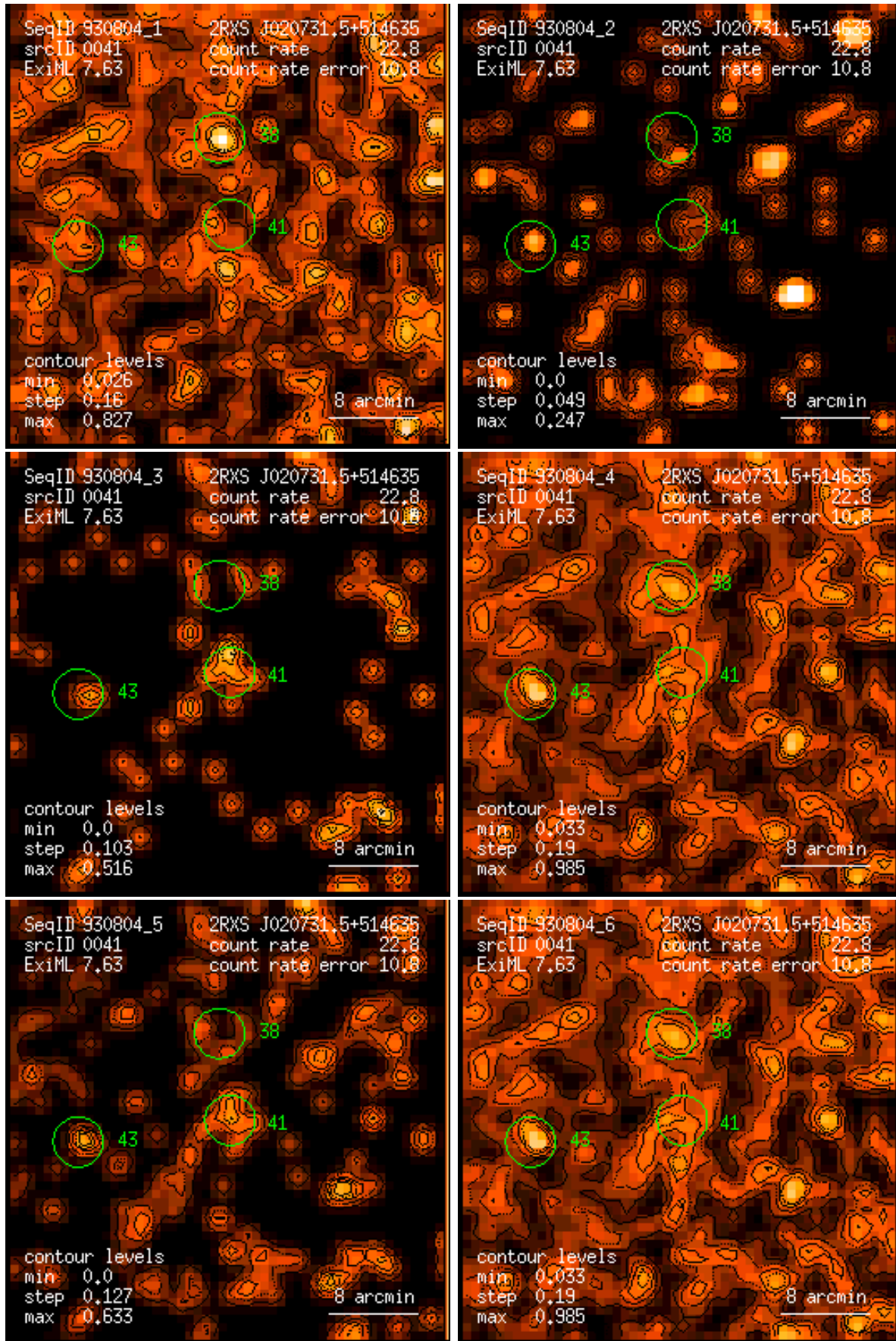
Figure 41: RASS 930804: detection 0041: band rate images, Gaussian filter: (1) PSPC channels 11 – 41, (2) 52 – 90, (3) 91 – 201, (4) 11 – 235, (5) 52 – 201, (6) 11 – 201. Broad band rates in counts/ks. Band rate contour levels in counts/ks/arcmin 2 .
