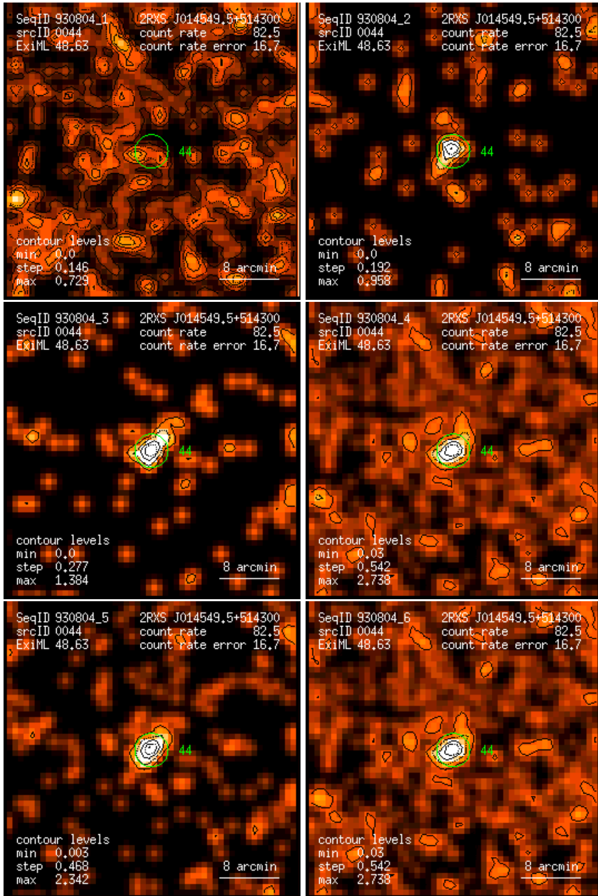
Figure 44: RASS 930804: detection 0044: band rate images, Gaussian filter: (1) PSPC channels 11 – 41, (2) 52 – 90, (3) 91 – 201, (4) 11 – 235, (5) 52 – 201, (6) 11 – 201. Broad band rates in counts/ks. Band rate contour levels in counts/ks/arcmin 2 .
