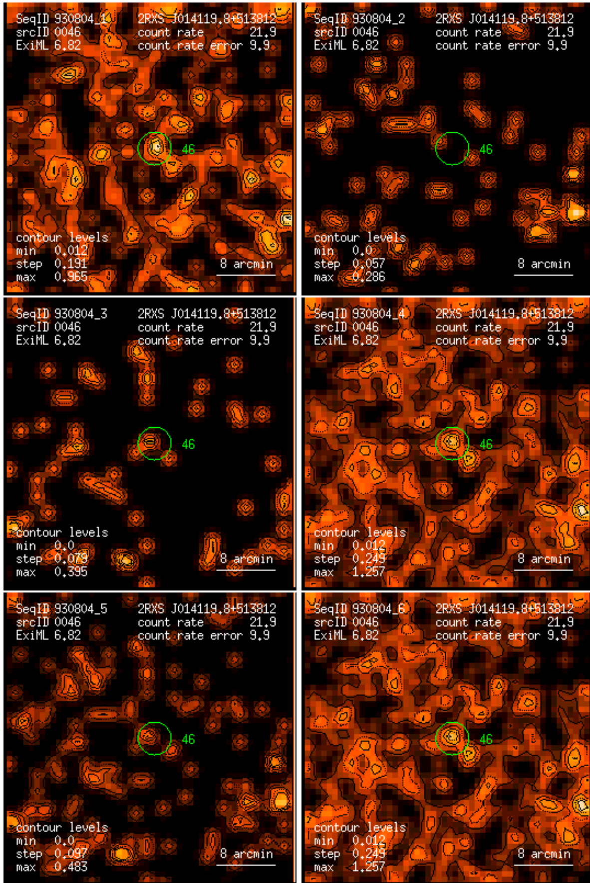
Figure 46: RASS 930804: detection 0046: band rate images, Gaussian filter: (1) PSPC channels 11 – 41, (2) 52 – 90, (3) 91 – 201, (4) 11 – 235, (5) 52 – 201, (6) 11 – 201. Broad band rates in counts/ks. Band rate contour levels in counts/ks/arcmin 2 .
