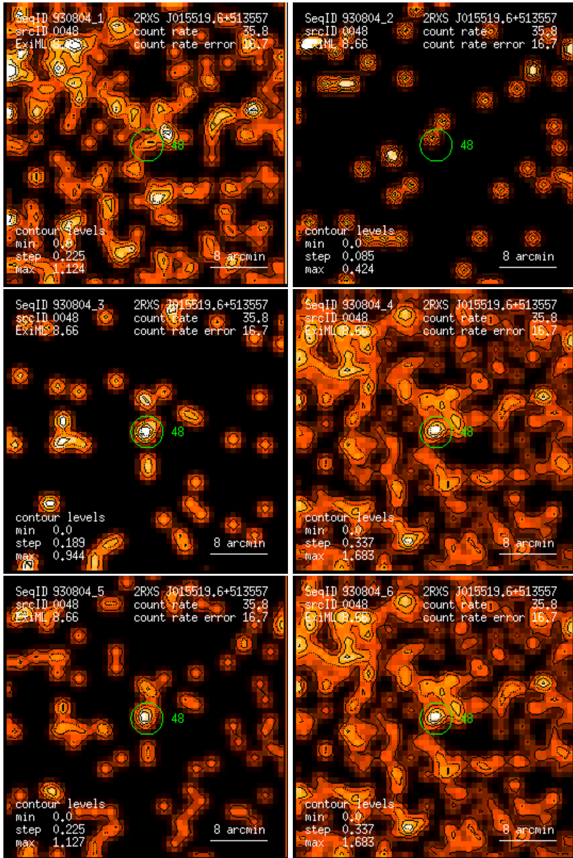
Figure 48: RASS 930804: detection 0048: band rate images, Gaussian filter: (1) PSPC channels 11 – 41, (2) 52 – 90, (3) 91 – 201, (4) 11 – 235, (5) 52 – 201, (6) 11 – 201. Broad band rates in counts/ks. Band rate contour levels in counts/ks/arcmin 2 .
