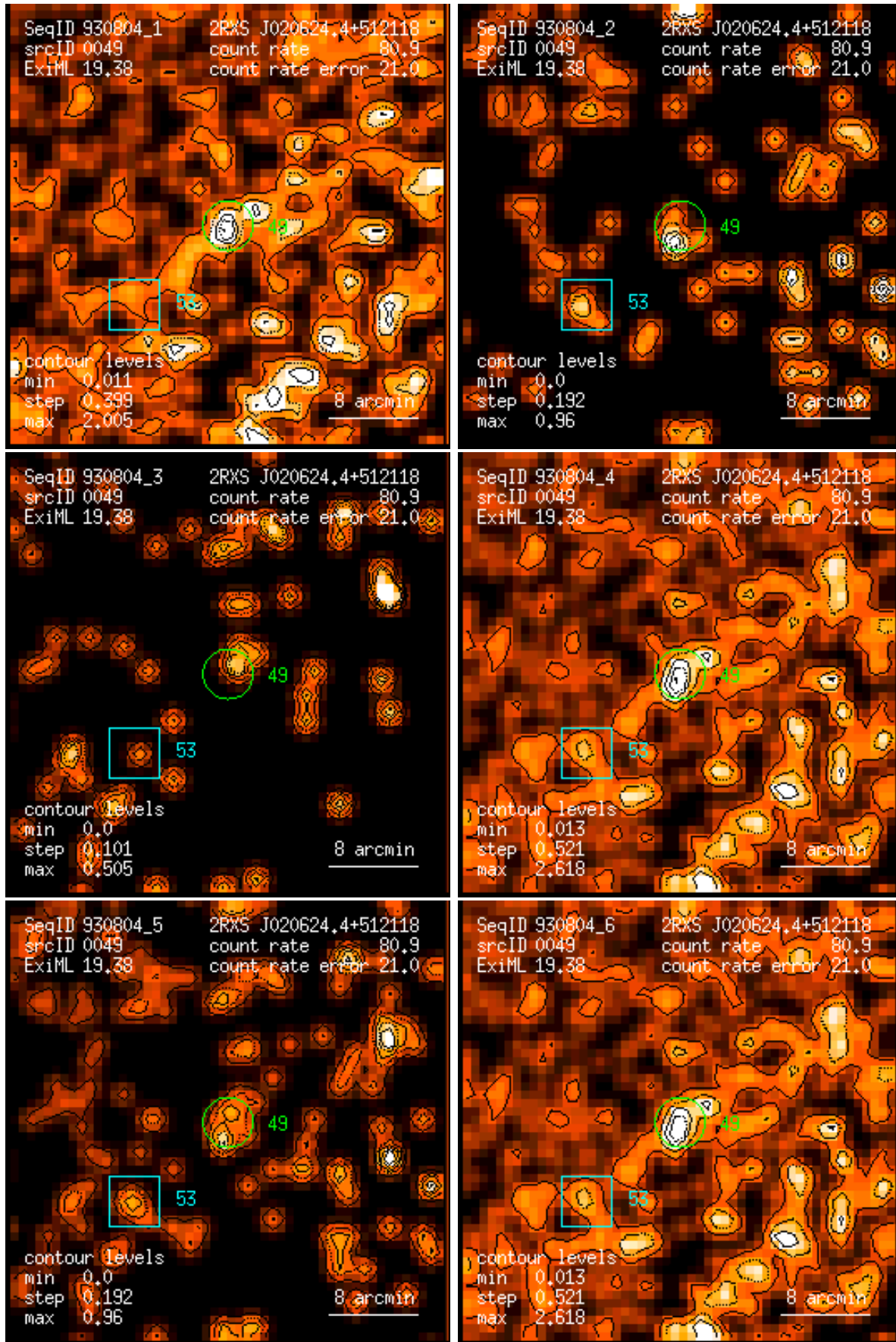
Figure 49: RASS 930804: detection 0049: band rate images, Gaussian filter: (1) PSPC channels 11 – 41, (2) 52 – 90, (3) 91 – 201, (4) 11 – 235, (5) 52 – 201, (6) 11 – 201. Broad band rates in counts/ks. Band rate contour levels in counts/ks/arcmin 2 .
