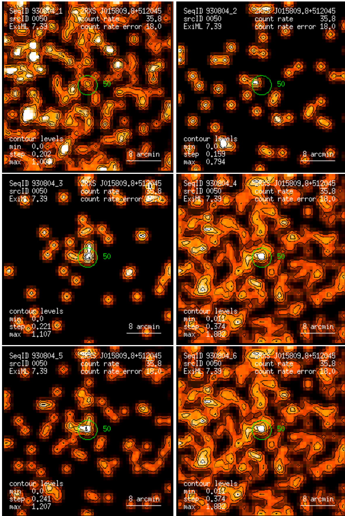
Figure 50: RASS 930804: detection 0050: band rate images, Gaussian filter: (1) PSPC channels 11 – 41, (2) 52 – 90, (3) 91 – 201, (4) 11 – 235, (5) 52 – 201, (6) 11 – 201. Broad band rates in counts/ks. Band rate contour levels in counts/ks/arcmin 2 .
