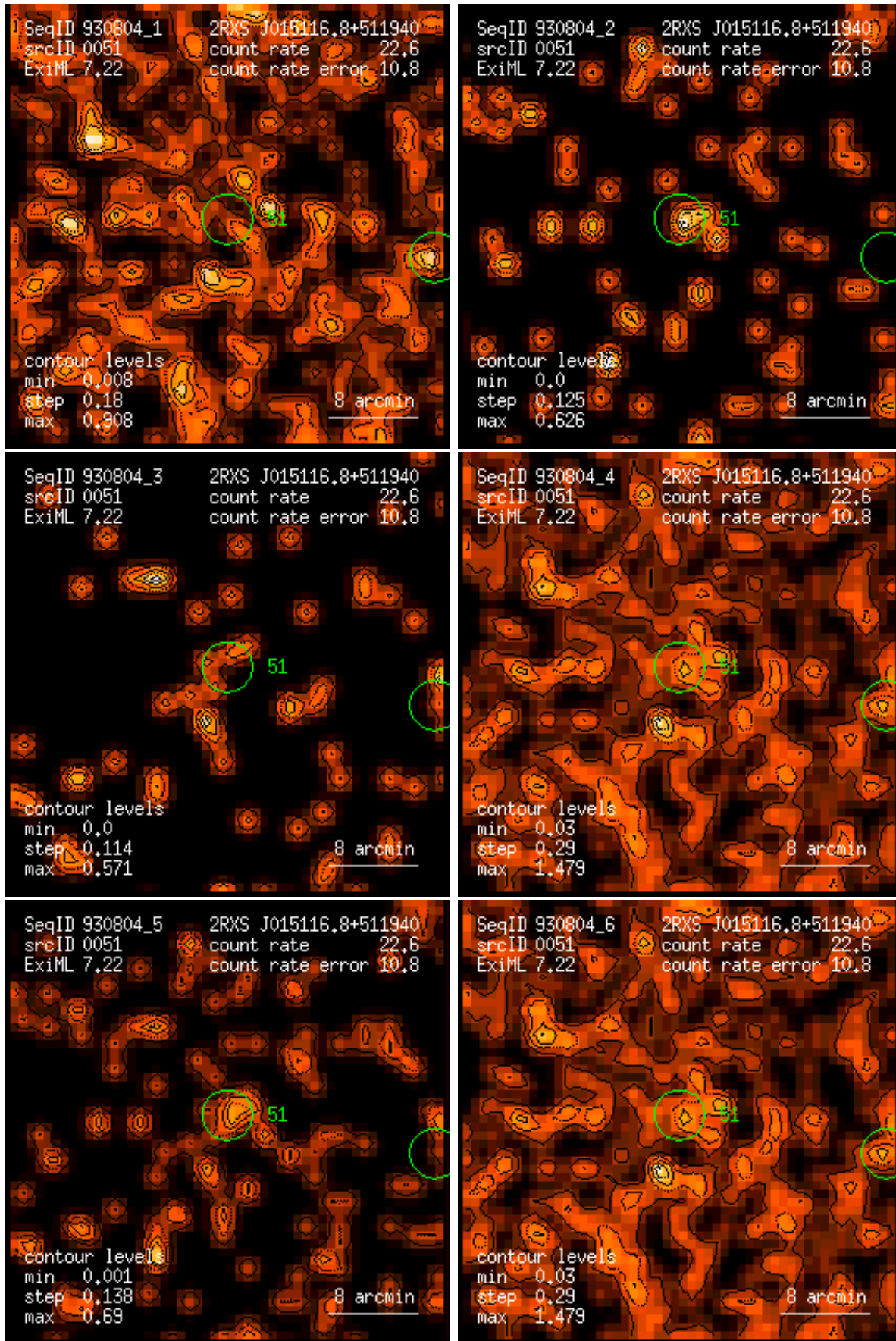
Figure 51: RASS 930804: detection 0051: band rate images, Gaussian filter: (1) PSPC channels 11 – 41, (2) 52 – 90, (3) 91 – 201, (4) 11 – 235, (5) 52 – 201, (6) 11 – 201. Broad band rates in counts/ks. Band rate contour levels in counts/ks/arcmin 2 .
