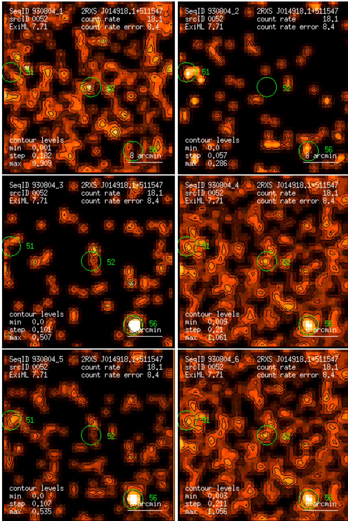
Figure 52: RASS 930804: detection 0052: band rate images, Gaussian filter: (1) PSPC channels 11 – 41, (2) 52 – 90, (3) 91 – 201, (4) 11 – 235, (5) 52 – 201, (6) 11 – 201. Broad band rates in counts/ks. Band rate contour levels in counts/ks/arcmin 2 .
