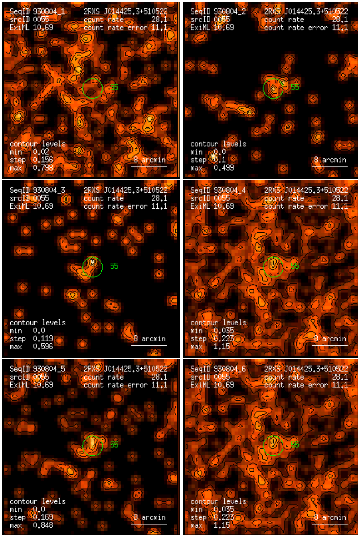
Figure 55: RASS 930804: detection 0055: band rate images, Gaussian filter: (1) PSPC channels 11 – 41, (2) 52 – 90, (3) 91 – 201, (4) 11 – 235, (5) 52 – 201, (6) 11 – 201. Broad band rates in counts/ks. Band rate contour levels in counts/ks/arcmin 2 .
