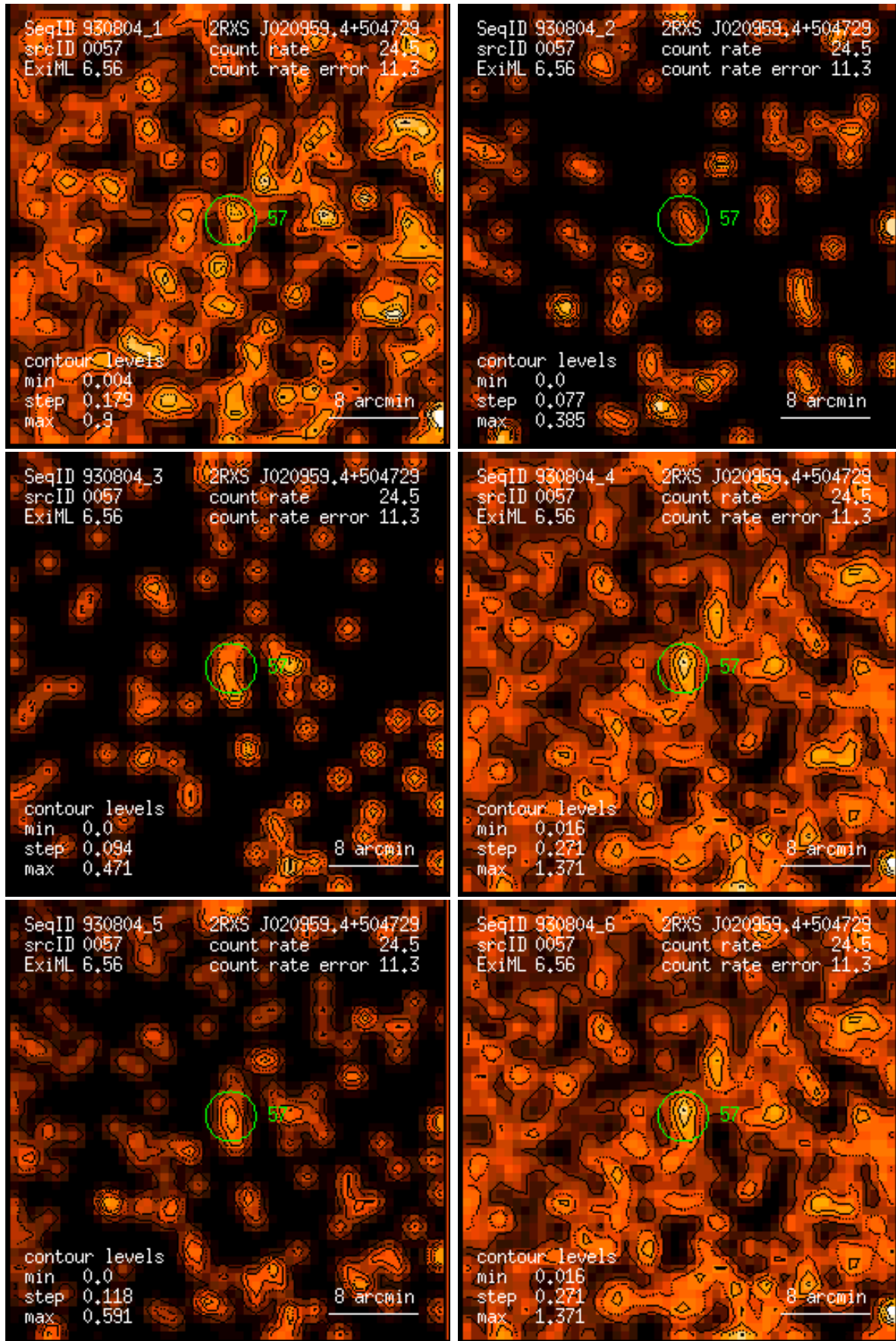
Figure 57: RASS 930804: detection 0057: band rate images, Gaussian filter: (1) PSPC channels 11 – 41, (2) 52 – 90, (3) 91 – 201, (4) 11 – 235, (5) 52 – 201, (6) 11 – 201. Broad band rates in counts/ks. Band rate contour levels in counts/ks/arcmin 2 .
