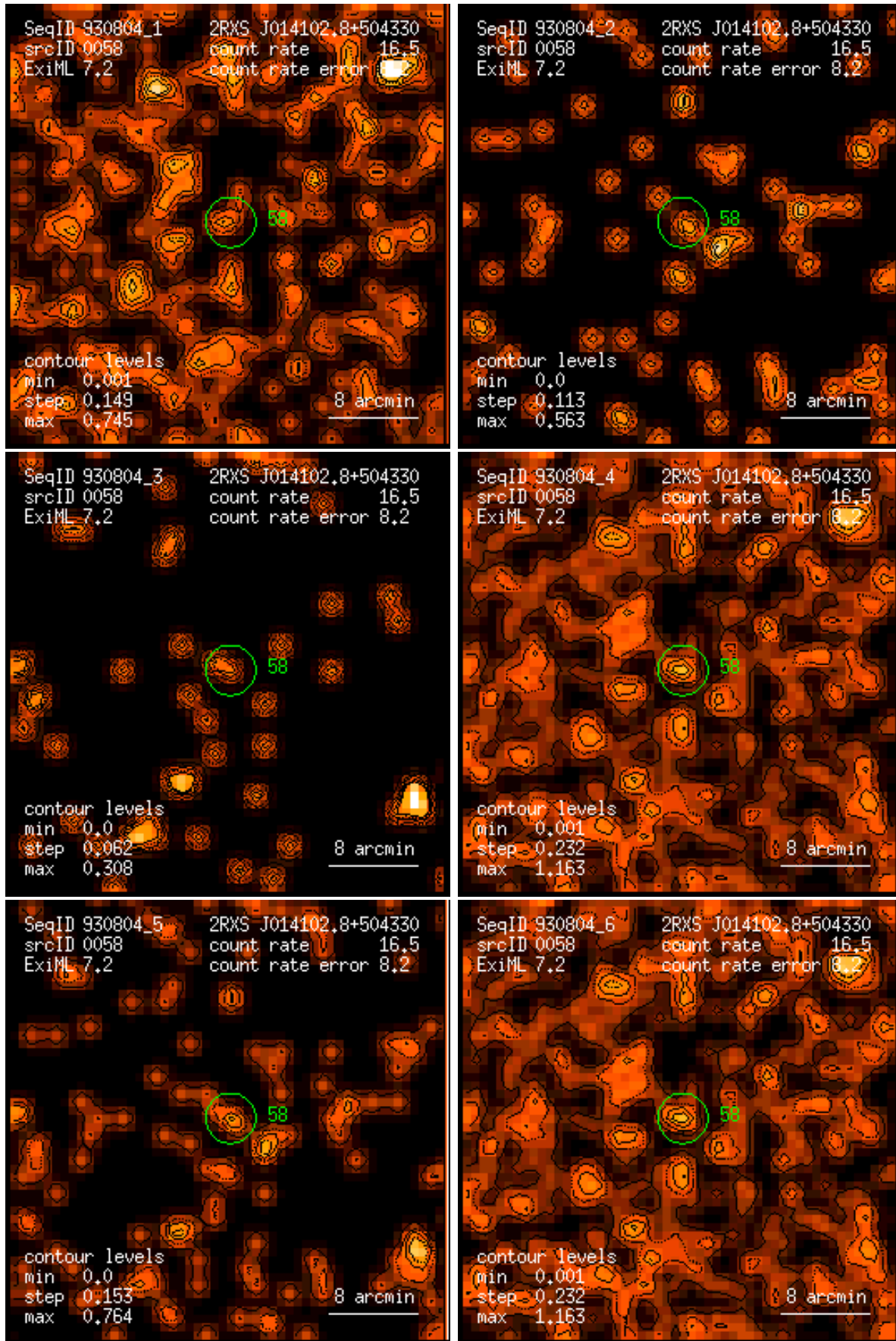
Figure 58: RASS 930804: detection 0058: band rate images, Gaussian filter: (1) PSPC channels 11 – 41, (2) 52 – 90, (3) 91 – 201, (4) 11 – 235, (5) 52 – 201, (6) 11 – 201. Broad band rates in counts/ks. Band rate contour levels in counts/ks/arcmin 2 .
