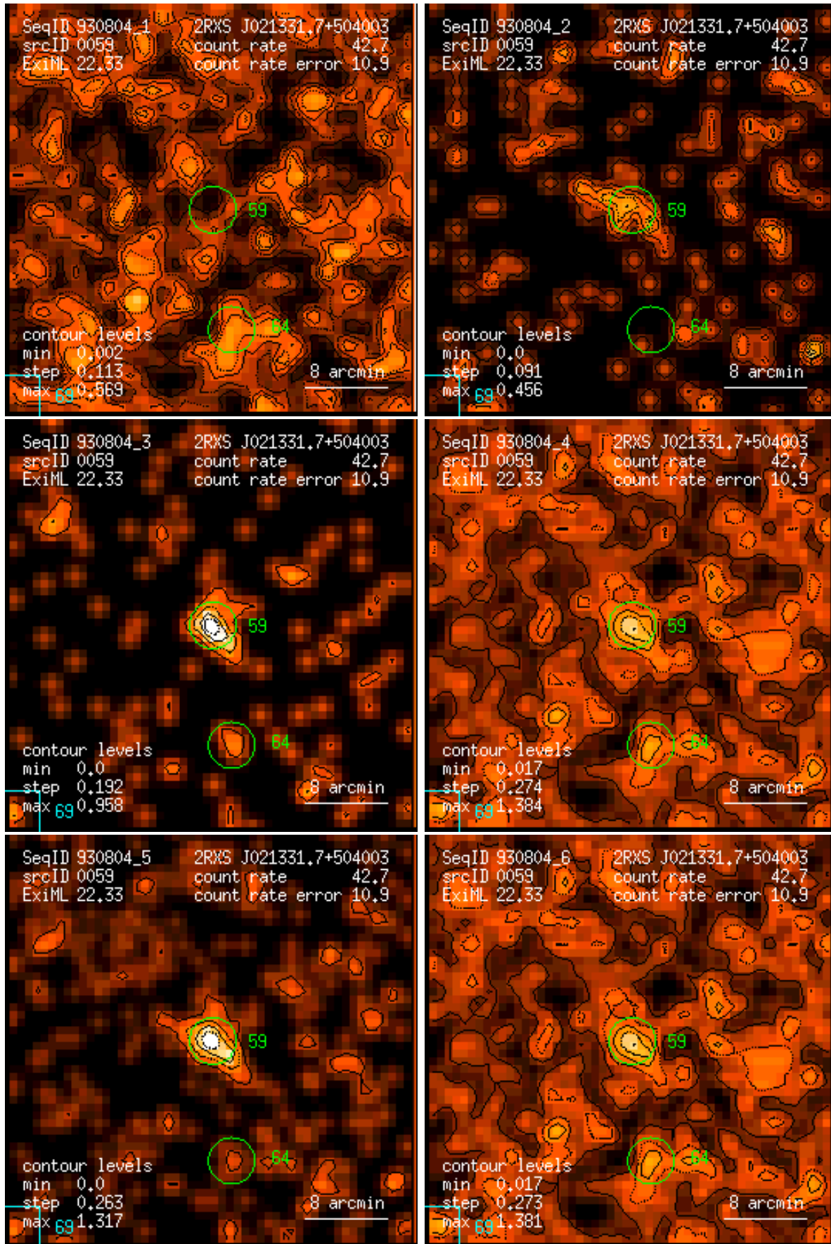
Figure 59: RASS 930804: detection 0059: band rate images, Gaussian filter: (1) PSPC channels 11 – 41, (2) 52 – 90, (3) 91 – 201, (4) 11 – 235, (5) 52 – 201, (6) 11 – 201. Broad band rates in counts/ks. Band rate contour levels in counts/ks/arcmin 2 .
