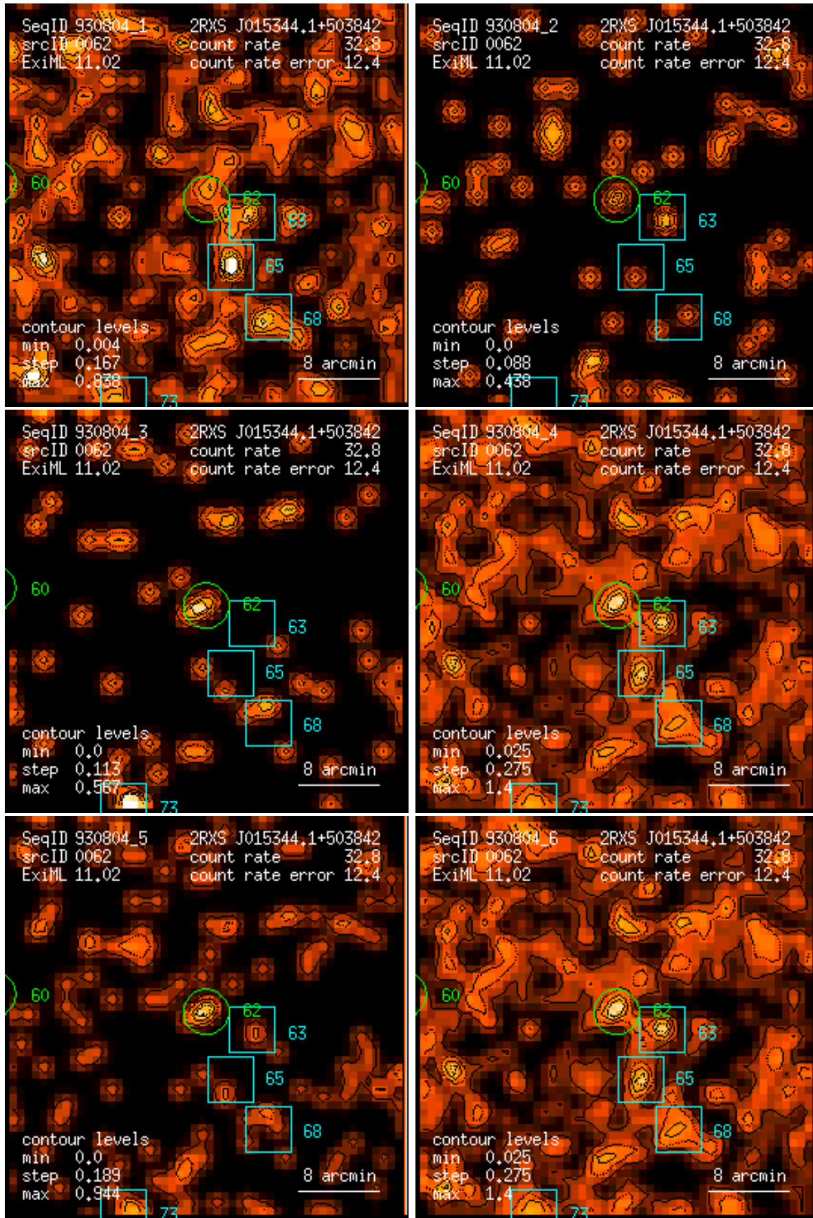
Figure 62: RASS 930804: detection 0062: band rate images, Gaussian filter: (1) PSPC channels 11 – 41, (2) 52 – 90, (3) 91 – 201, (4) 11 – 235, (5) 52 – 201, (6) 11 – 201. Broad band rates in counts/ks. Band rate contour levels in counts/ks/arcmin 2 .
