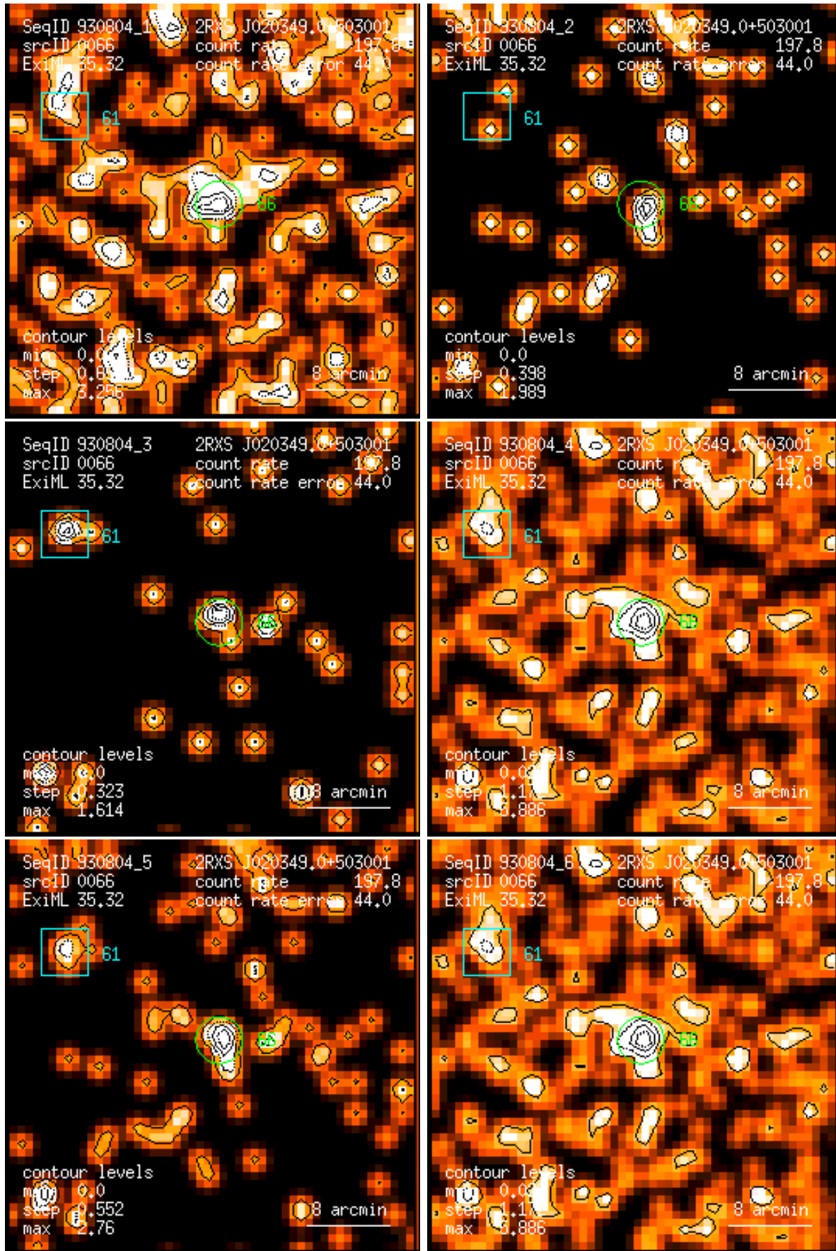
Figure 66: RASS 930804: detection 0066: band rate images, Gaussian filter: (1) PSPC channels 11 – 41, (2) 52 – 90, (3) 91 – 201, (4) 11 – 235, (5) 52 – 201, (6) 11 – 201. Broad band rates in counts/ks. Band rate contour levels in counts/ks/arcmin 2 .
