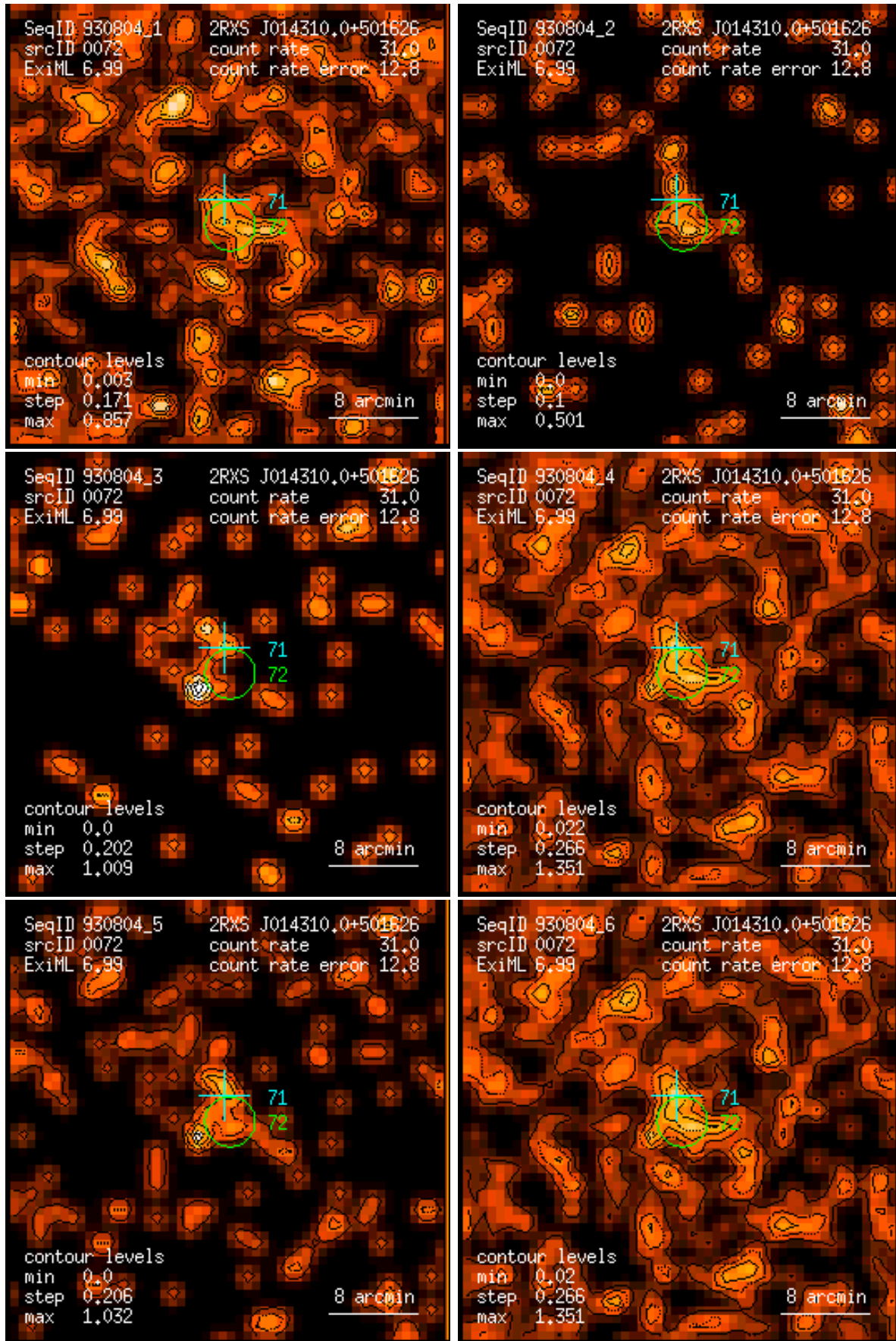
Figure 72: RASS 930804: detection 0072: band rate images, Gaussian filter: (1) PSPC channels 11 – 41, (2) 52 – 90, (3) 91 – 201, (4) 11 – 235, (5) 52 – 201, (6) 11 – 201. Broad band rates in counts/ks. Band rate contour levels in counts/ks/arcmin 2 .
