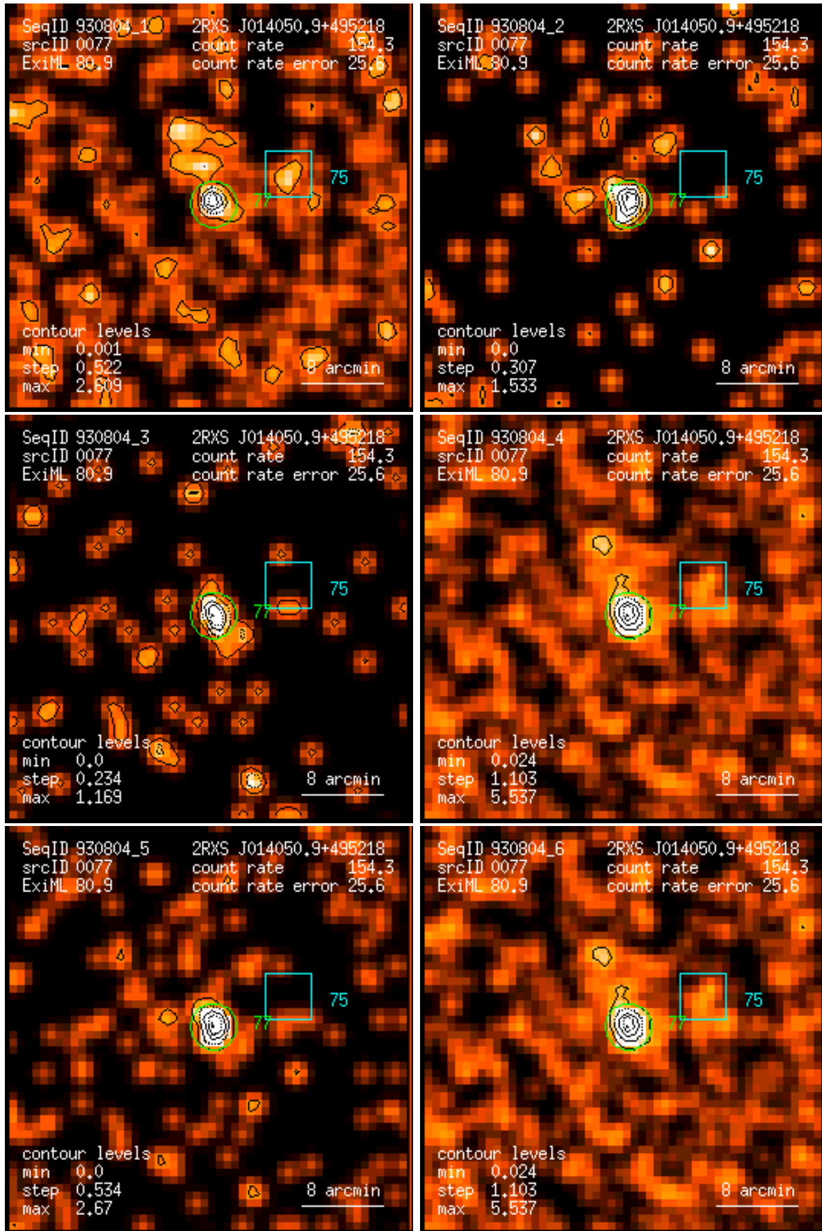
Figure 77: RASS 930804: detection 0077: band rate images, Gaussian filter: (1) PSPC channels 11 – 41, (2) 52 – 90, (3) 91 – 201, (4) 11 – 235, (5) 52 – 201, (6) 11 – 201. Broad band rates in counts/ks. Band rate contour levels in counts/ks/arcmin 2 .
