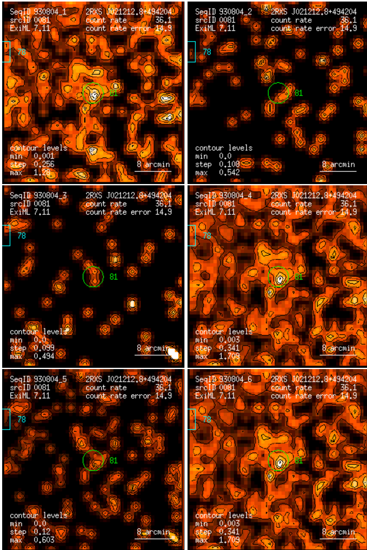
Figure 81: RASS 930804: detection 0081: band rate images, Gaussian filter: (1) PSPC channels 11 – 41, (2) 52 – 90, (3) 91 – 201, (4) 11 – 235, (5) 52 – 201, (6) 11 – 201. Broad band rates in counts/ks. Band rate contour levels in counts/ks/arcmin 2 .
