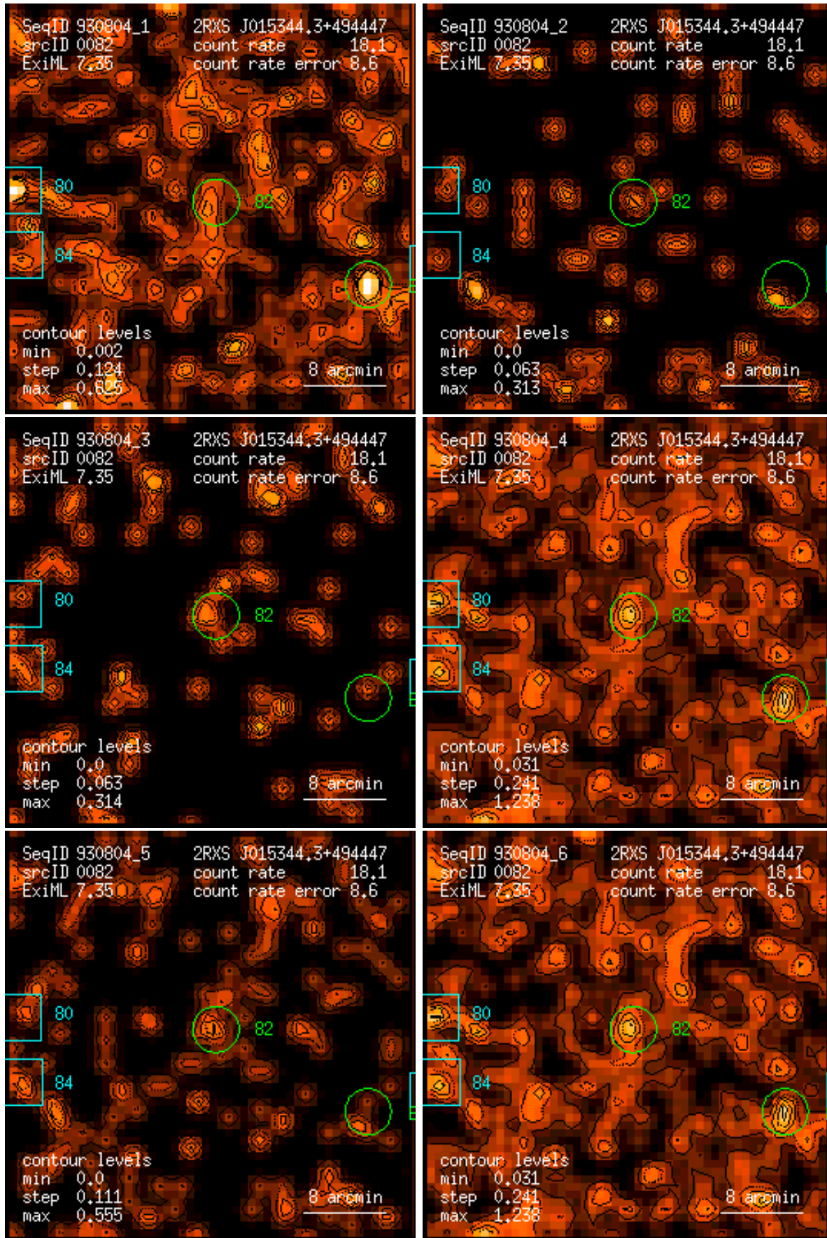
Figure 82: RASS 930804: detection 0082: band rate images, Gaussian filter: (1) PSPC channels 11 – 41, (2) 52 – 90, (3) 91 – 201, (4) 11 – 235, (5) 52 – 201, (6) 11 – 201. Broad band rates in counts/ks. Band rate contour levels in counts/ks/arcmin 2 .
