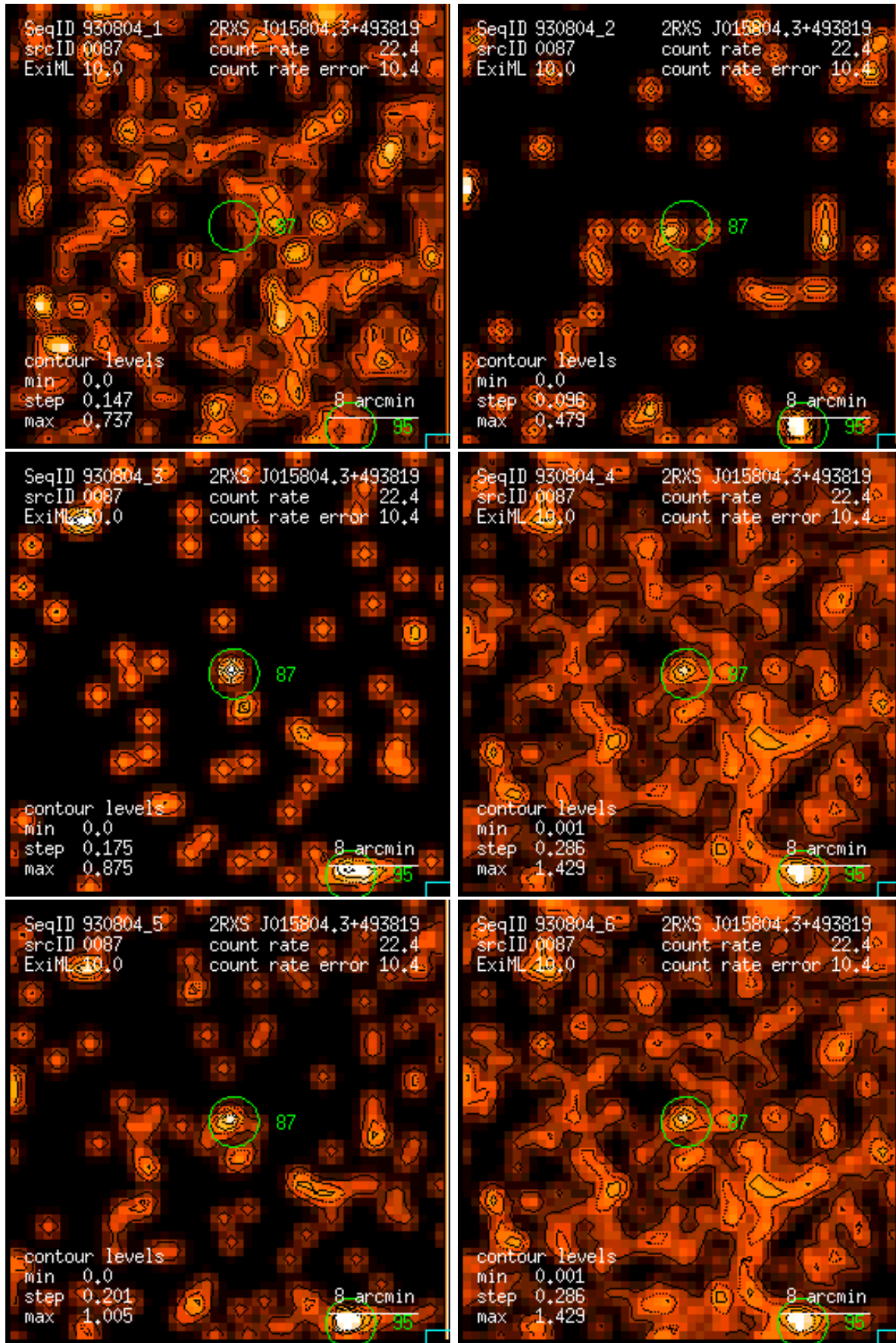
Figure 87: RASS 930804: detection 0087: band rate images, Gaussian filter: (1) PSPC channels 11 – 41, (2) 52 – 90, (3) 91 – 201, (4) 11 – 235, (5) 52 – 201, (6) 11 – 201. Broad band rates in counts/ks. Band rate contour levels in counts/ks/arcmin 2 .
