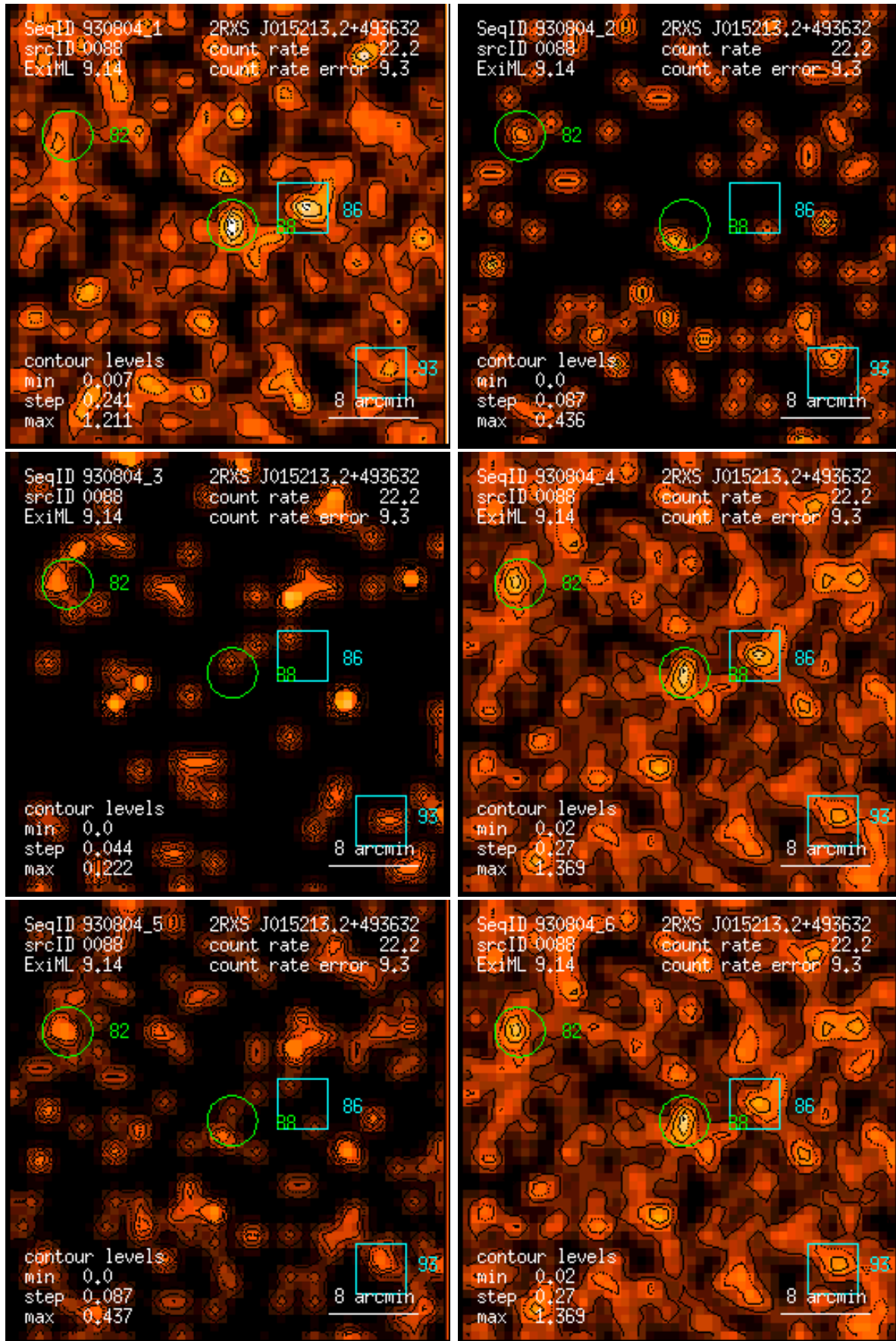
Figure 88: RASS 930804: detection 0088: band rate images, Gaussian filter: (1) PSPC channels 11 – 41, (2) 52 – 90, (3) 91 – 201, (4) 11 – 235, (5) 52 – 201, (6) 11 – 201. Broad band rates in counts/ks. Band rate contour levels in counts/ks/arcmin 2 .
