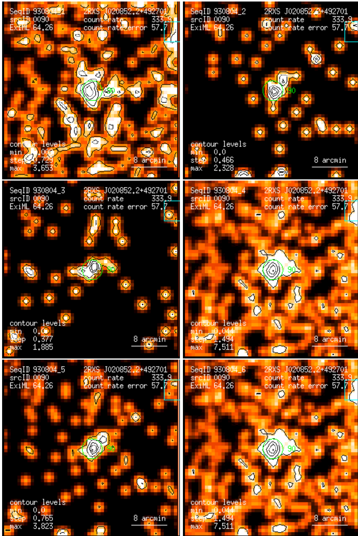
Figure 90: RASS 930804: detection 0090: band rate images, Gaussian filter: (1) PSPC channels 11 – 41, (2) 52 – 90, (3) 91 – 201, (4) 11 – 235, (5) 52 – 201, (6) 11 – 201. Broad band rates in counts/ks. Band rate contour levels in counts/ks/arcmin 2 .
