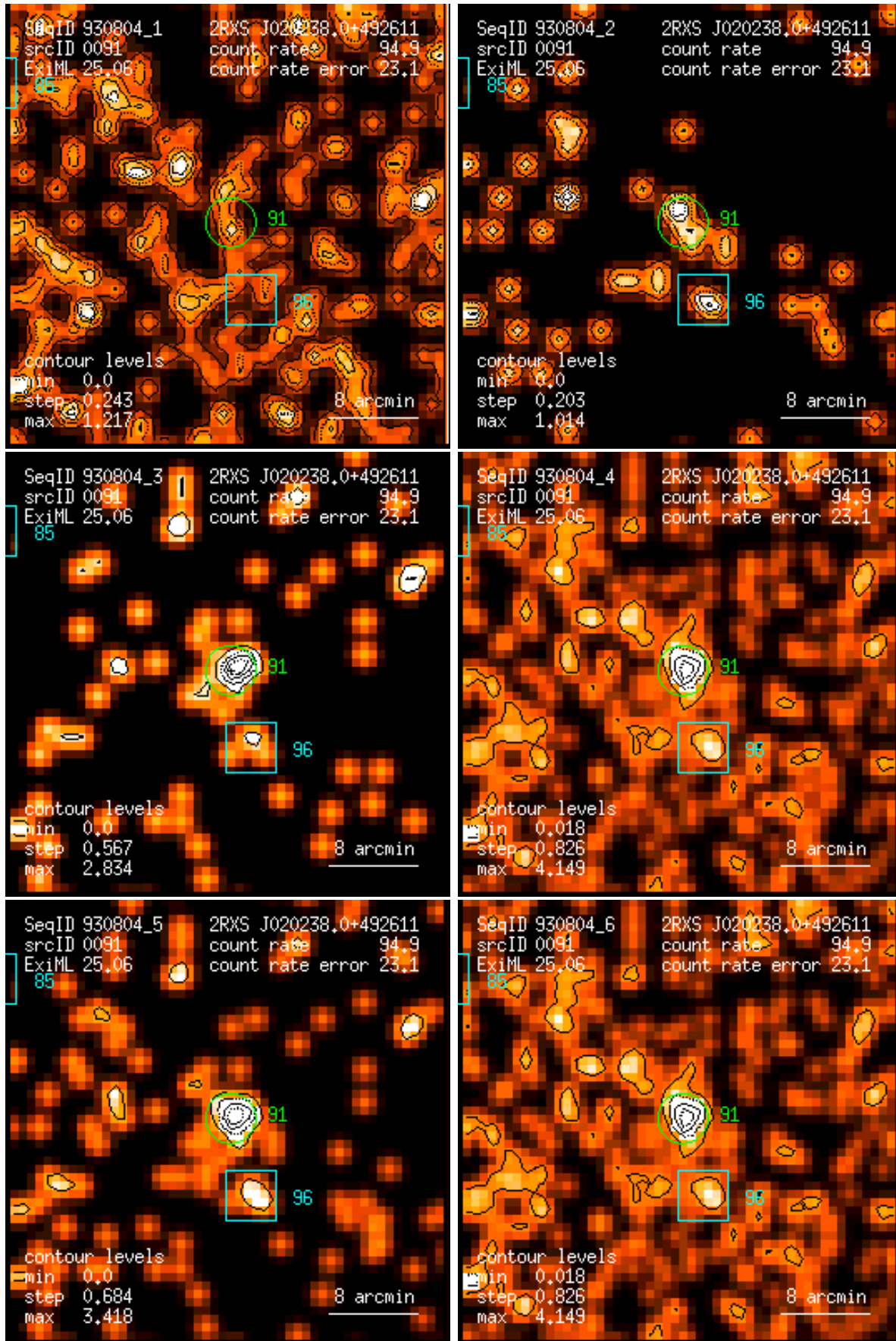
Figure 91: RASS 930804: detection 0091: band rate images, Gaussian filter: (1) PSPC channels 11 – 41, (2) 52 – 90, (3) 91 – 201, (4) 11 – 235, (5) 52 – 201, (6) 11 – 201. Broad band rates in counts/ks. Band rate contour levels in counts/ks/arcmin 2 .
