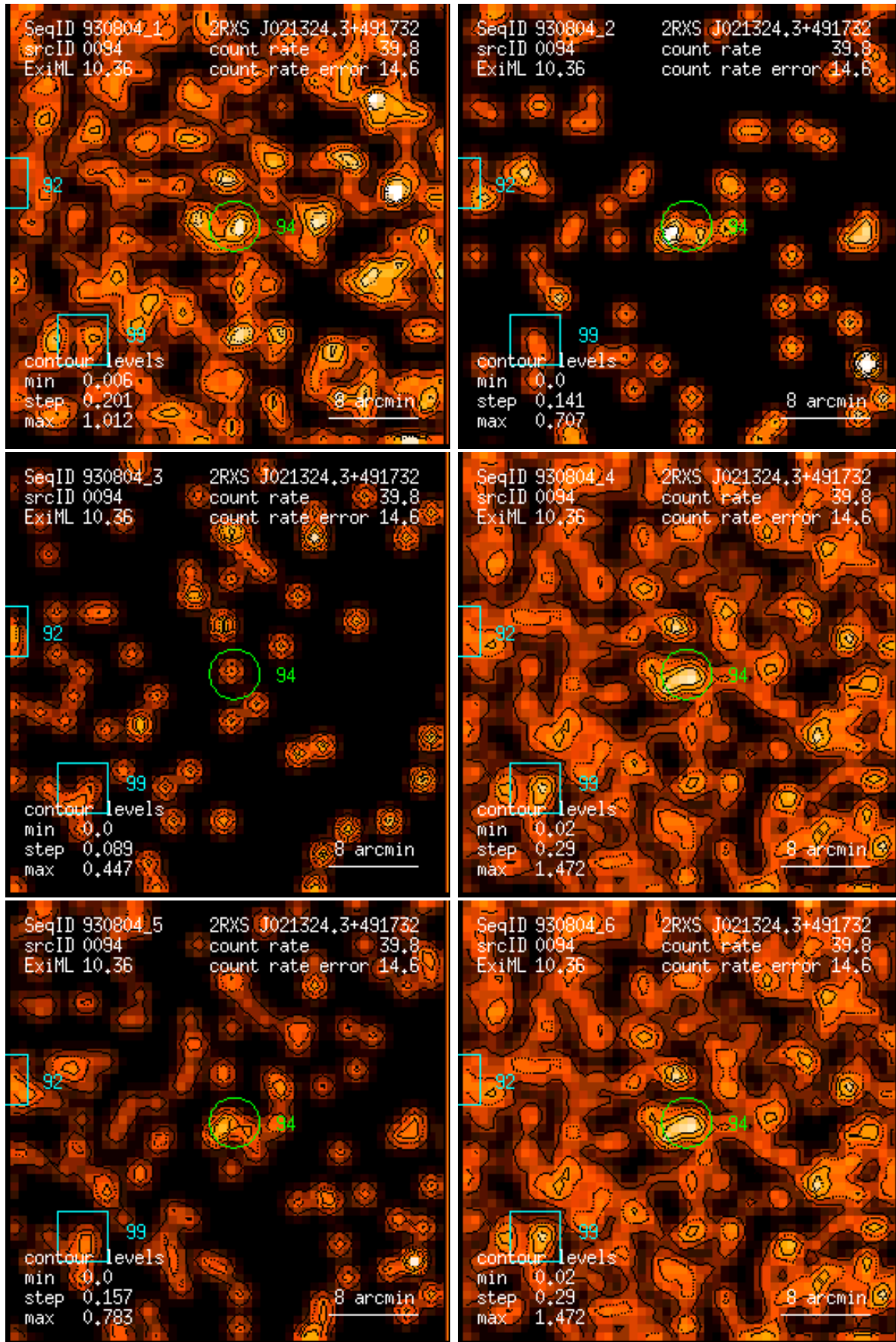
Figure 94: RASS 930804: detection 0094: band rate images, Gaussian filter: (1) PSPC channels 11 – 41, (2) 52 – 90, (3) 91 – 201, (4) 11 – 235, (5) 52 – 201, (6) 11 – 201. Broad band rates in counts/ks. Band rate contour levels in counts/ks/arcmin 2 .
