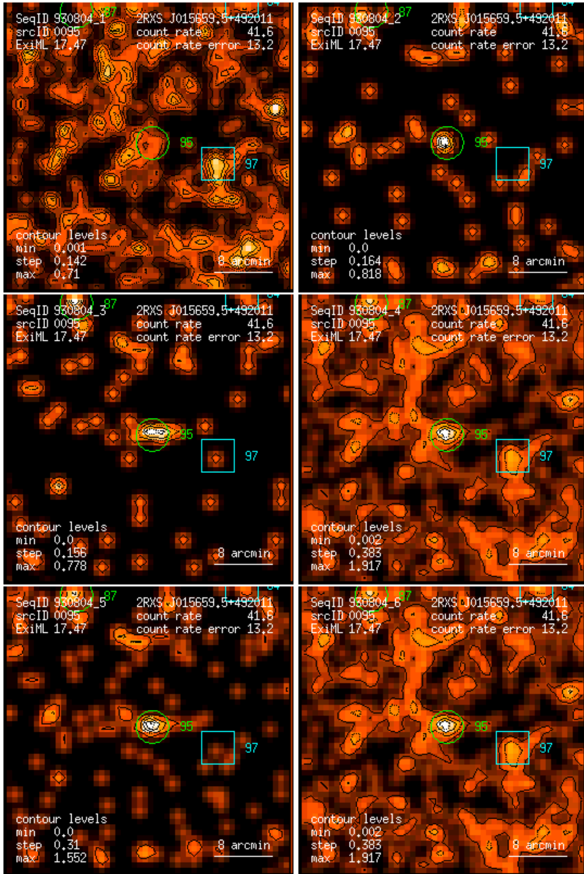
Figure 95: RASS 930804: detection 0095: band rate images, Gaussian filter: (1) PSPC channels 11 – 41, (2) 52 – 90, (3) 91 – 201, (4) 11 – 235, (5) 52 – 201, (6) 11 – 201. Broad band rates in counts/ks. Band rate contour levels in counts/ks/arcmin 2 .
