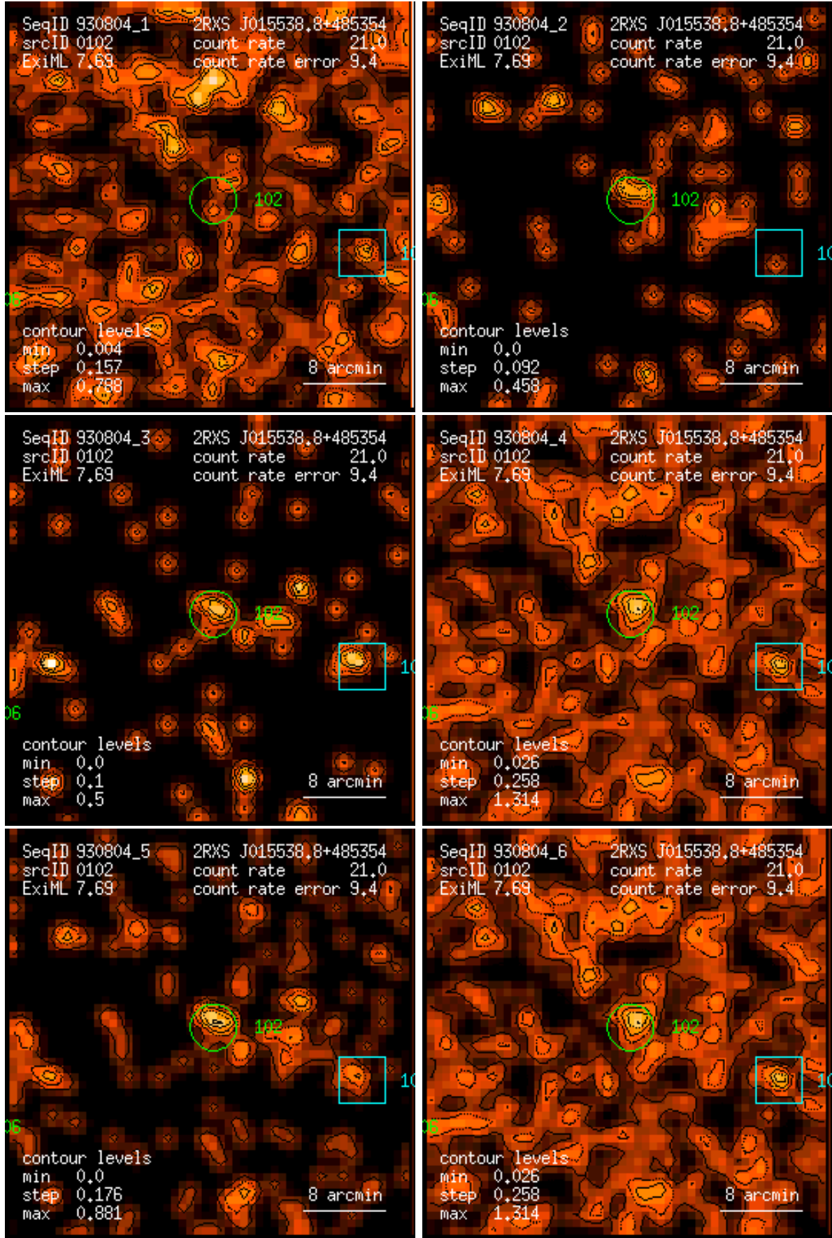
Figure 102: RASS 930804: detection 0102: band rate images, Gaussian filter: (1) PSPC channels 11 – 41, (2) 52 – 90, (3) 91 – 201, (4) 11 – 235, (5) 52 – 201, (6) 11 – 201. Broad band rates in counts/ks. Band rate contour levels in counts/ks/arcmin 2 .
