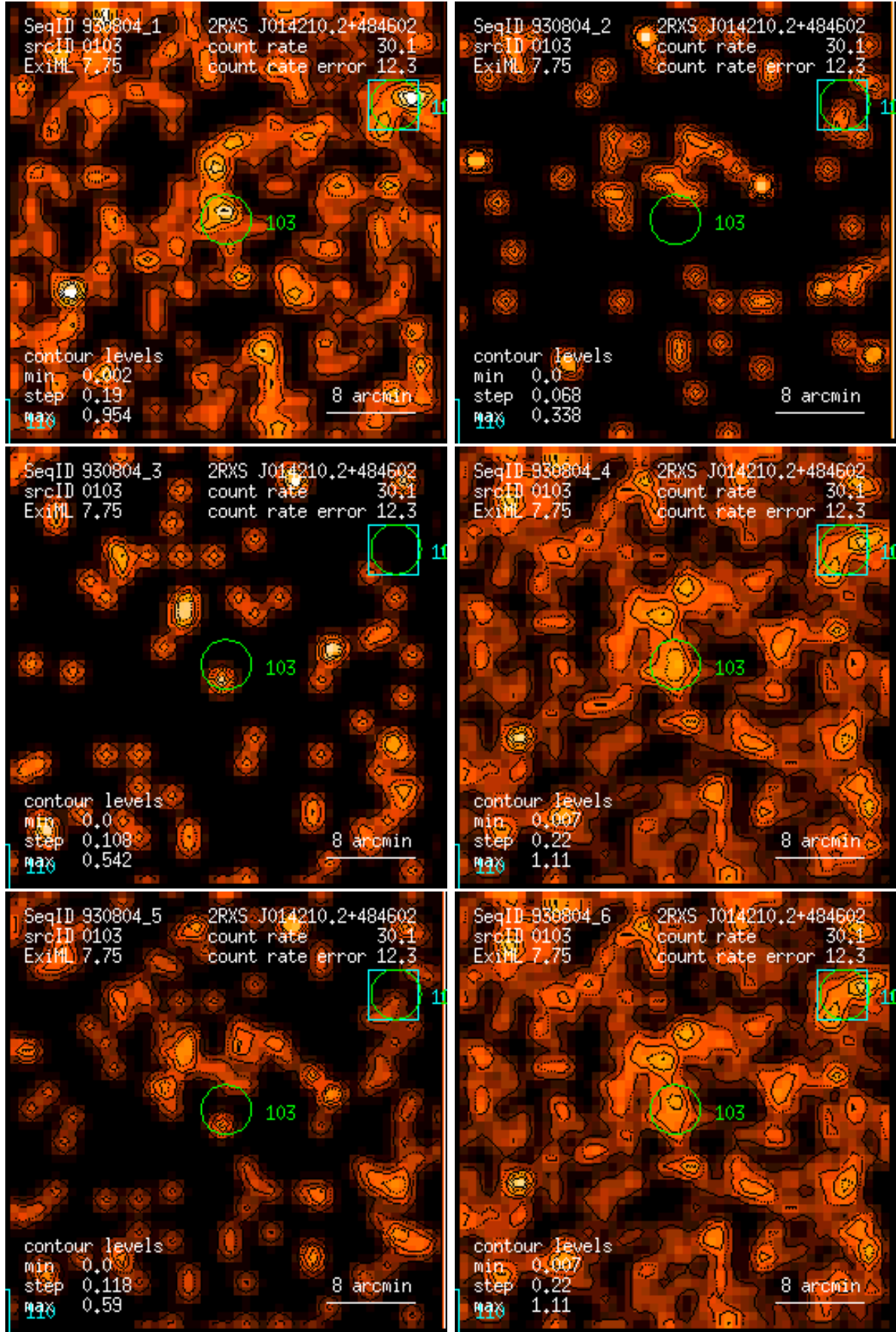
Figure 103: RASS 930804: detection 0103: band rate images, Gaussian filter: (1) PSPC channels 11 – 41, (2) 52 – 90, (3) 91 – 201, (4) 11 – 235, (5) 52 – 201, (6) 11 – 201. Broad band rates in counts/ks. Band rate contour levels in counts/ks/arcmin 2 .
