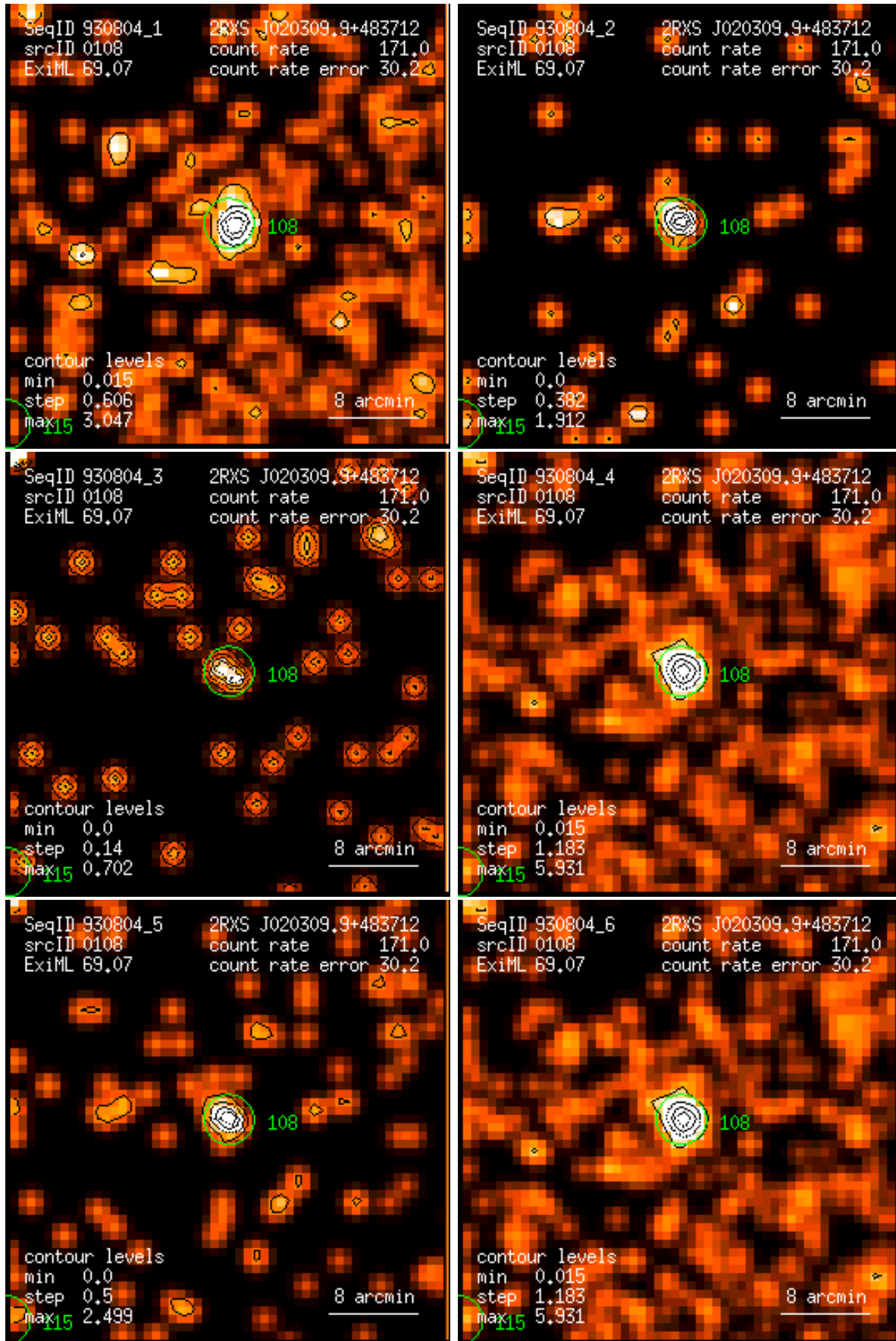
Figure 108: RASS 930804: detection 0108: band rate images, Gaussian filter: (1) PSPC channels 11 – 41, (2) 52 – 90, (3) 91 – 201, (4) 11 – 235, (5) 52 – 201, (6) 11 – 201. Broad band rates in counts/ks. Band rate contour levels in counts/ks/arcmin 2 .
