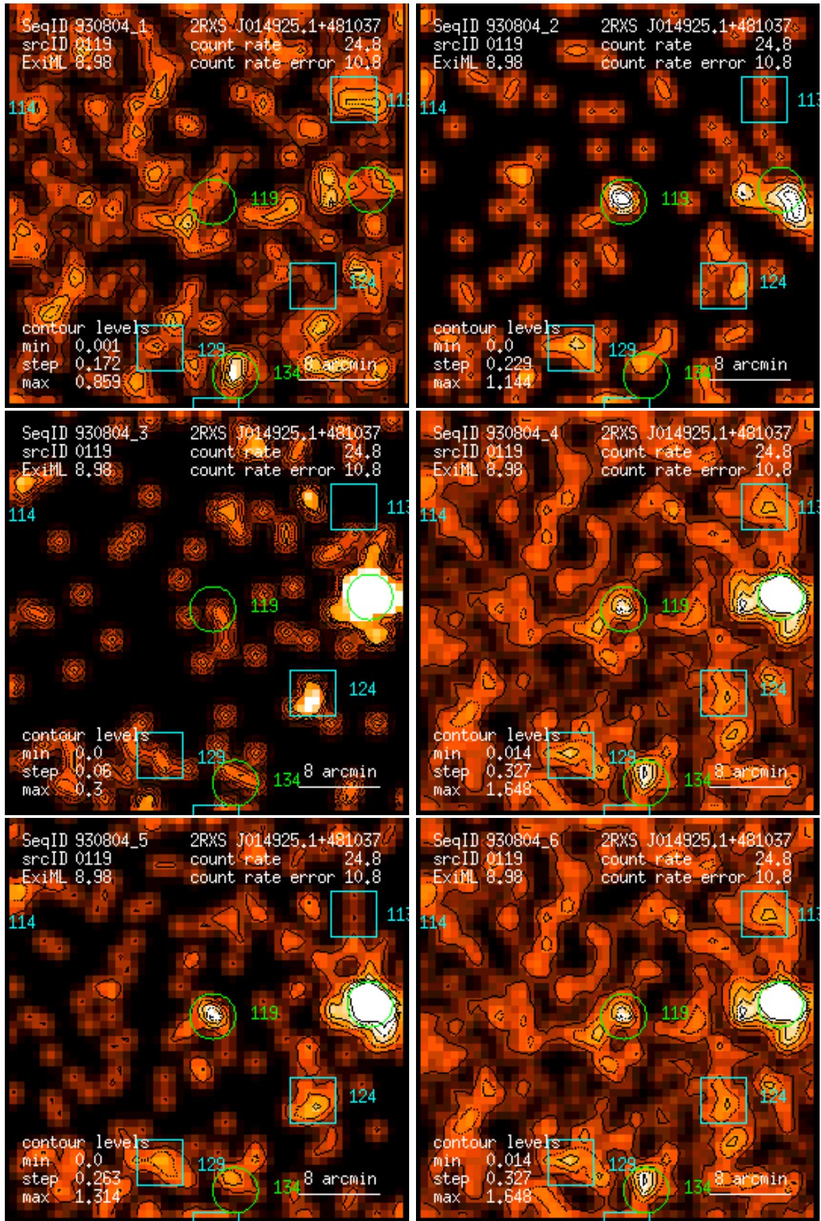
Figure 119: RASS 930804: detection 0119: band rate images, Gaussian filter: (1) PSPC channels 11 – 41, (2) 52 – 90, (3) 91 – 201, (4) 11 – 235, (5) 52 – 201, (6) 11 – 201. Broad band rates in counts/ks. Band rate contour levels in counts/ks/arcmin 2 .
