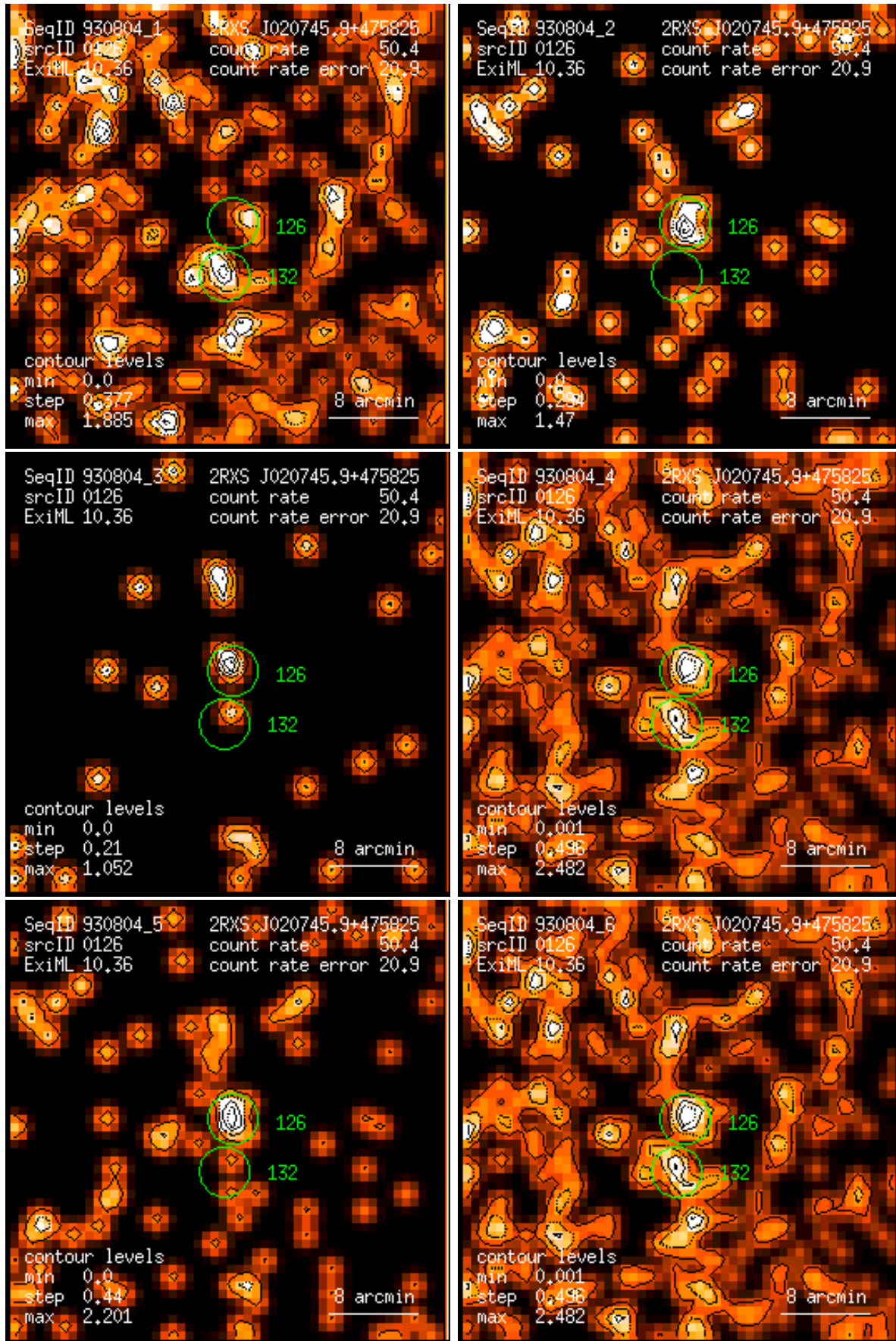
Figure 126: RASS 930804: detection 0126: band rate images, Gaussian filter: (1) PSPC channels 11 – 41, (2) 52 – 90, (3) 91 – 201, (4) 11 – 235, (5) 52 – 201, (6) 11 – 201. Broad band rates in counts/ks. Band rate contour levels in counts/ks/arcmin 2 .
