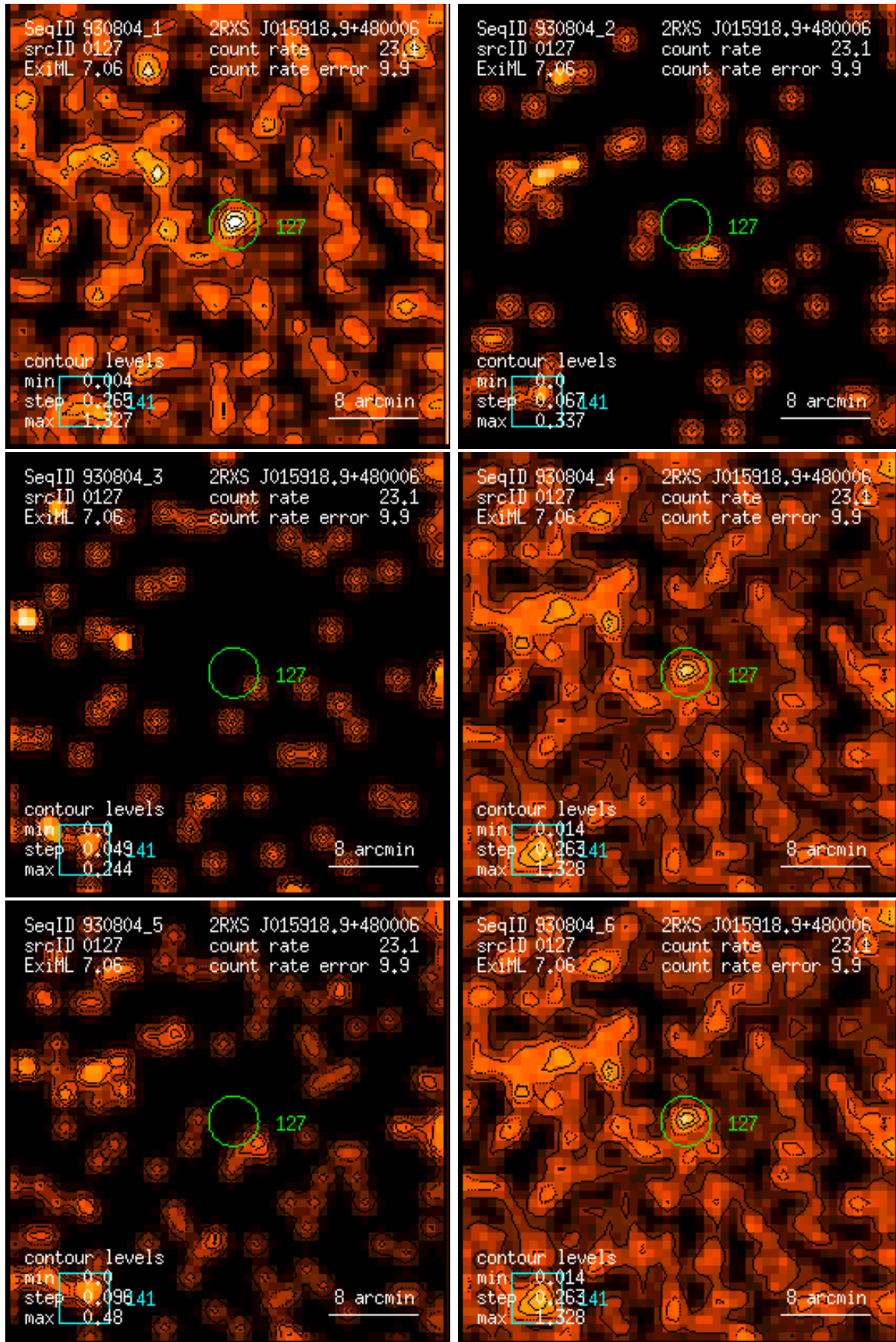
Figure 127: RASS 930804: detection 0127: band rate images, Gaussian filter: (1) PSPC channels 11 – 41, (2) 52 – 90, (3) 91 – 201, (4) 11 – 235, (5) 52 – 201, (6) 11 – 201. Broad band rates in counts/ks. Band rate contour levels in counts/ks/arcmin 2 .
