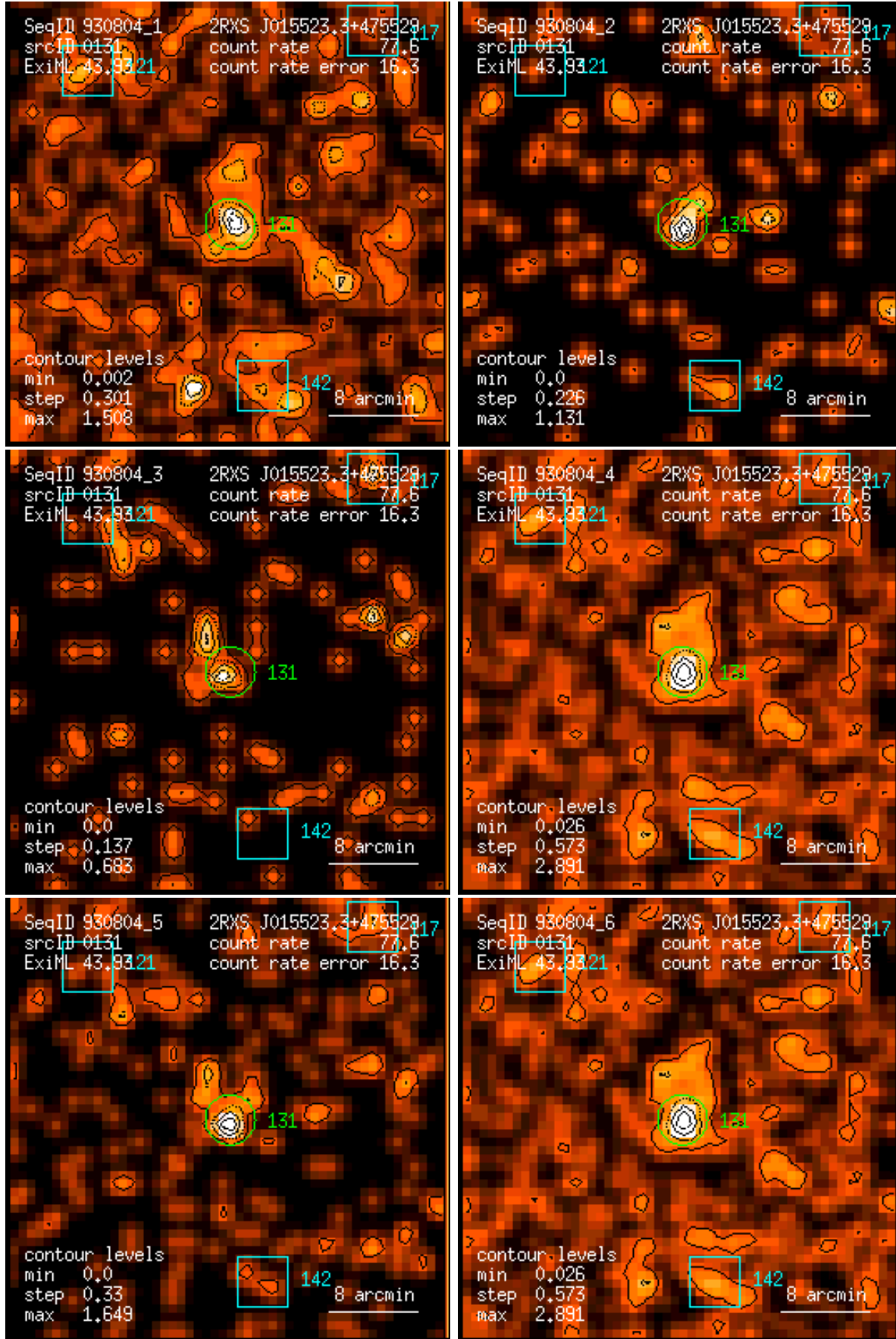
Figure 131: RASS 930804: detection 0131: band rate images, Gaussian filter: (1) PSPC channels 11 – 41, (2) 52 – 90, (3) 91 – 201, (4) 11 – 235, (5) 52 – 201, (6) 11 – 201. Broad band rates in counts/ks. Band rate contour levels in counts/ks/arcmin 2 .
