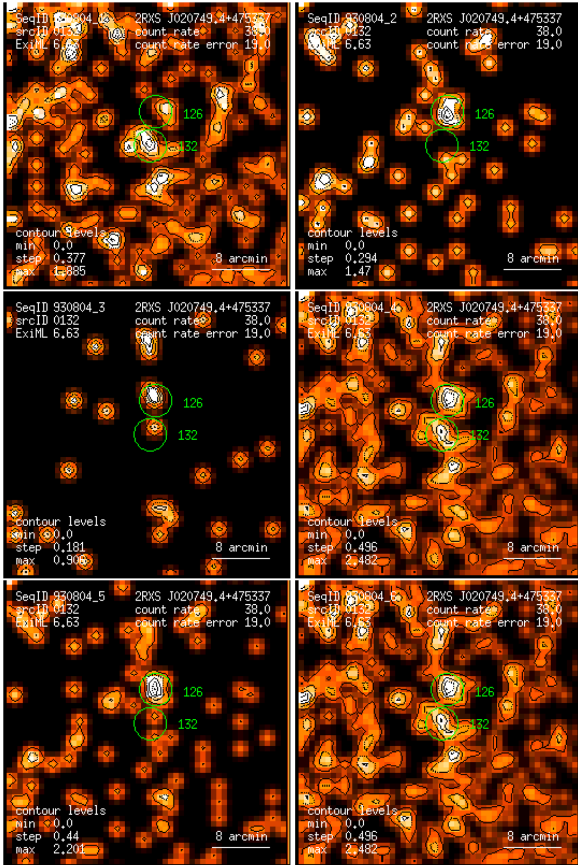
Figure 132: RASS 930804: detection 0132: band rate images, Gaussian filter: (1) PSPC channels 11 – 41, (2) 52 – 90, (3) 91 – 201, (4) 11 – 235, (5) 52 – 201, (6) 11 – 201. Broad band rates in counts/ks. Band rate contour levels in counts/ks/arcmin 2 .
