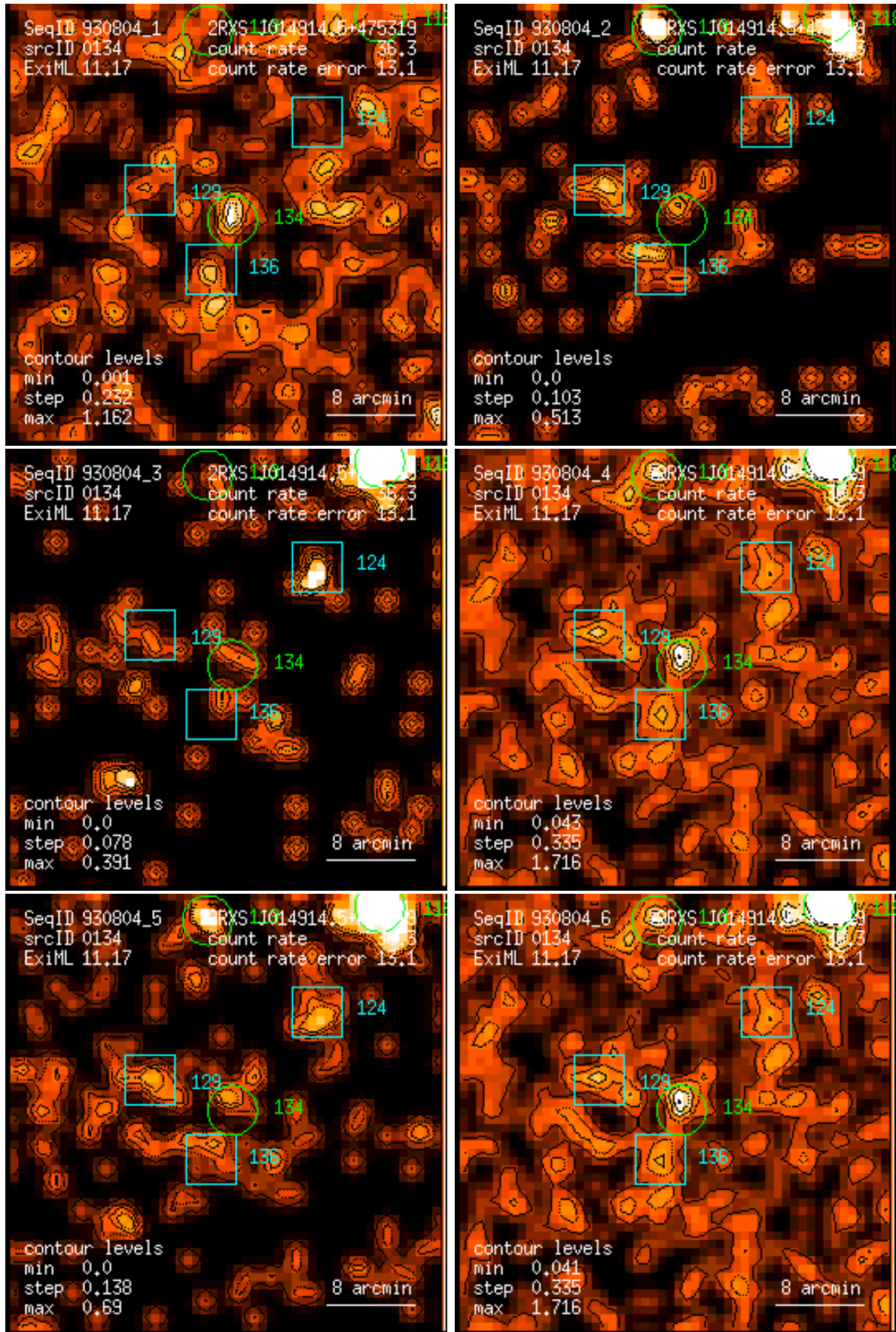
Figure 134: RASS 930804: detection 0134: band rate images, Gaussian filter: (1) PSPC channels 11 – 41, (2) 52 – 90, (3) 91 – 201, (4) 11 – 235, (5) 52 – 201, (6) 11 – 201. Broad band rates in counts/ks. Band rate contour levels in counts/ks/arcmin 2 .
