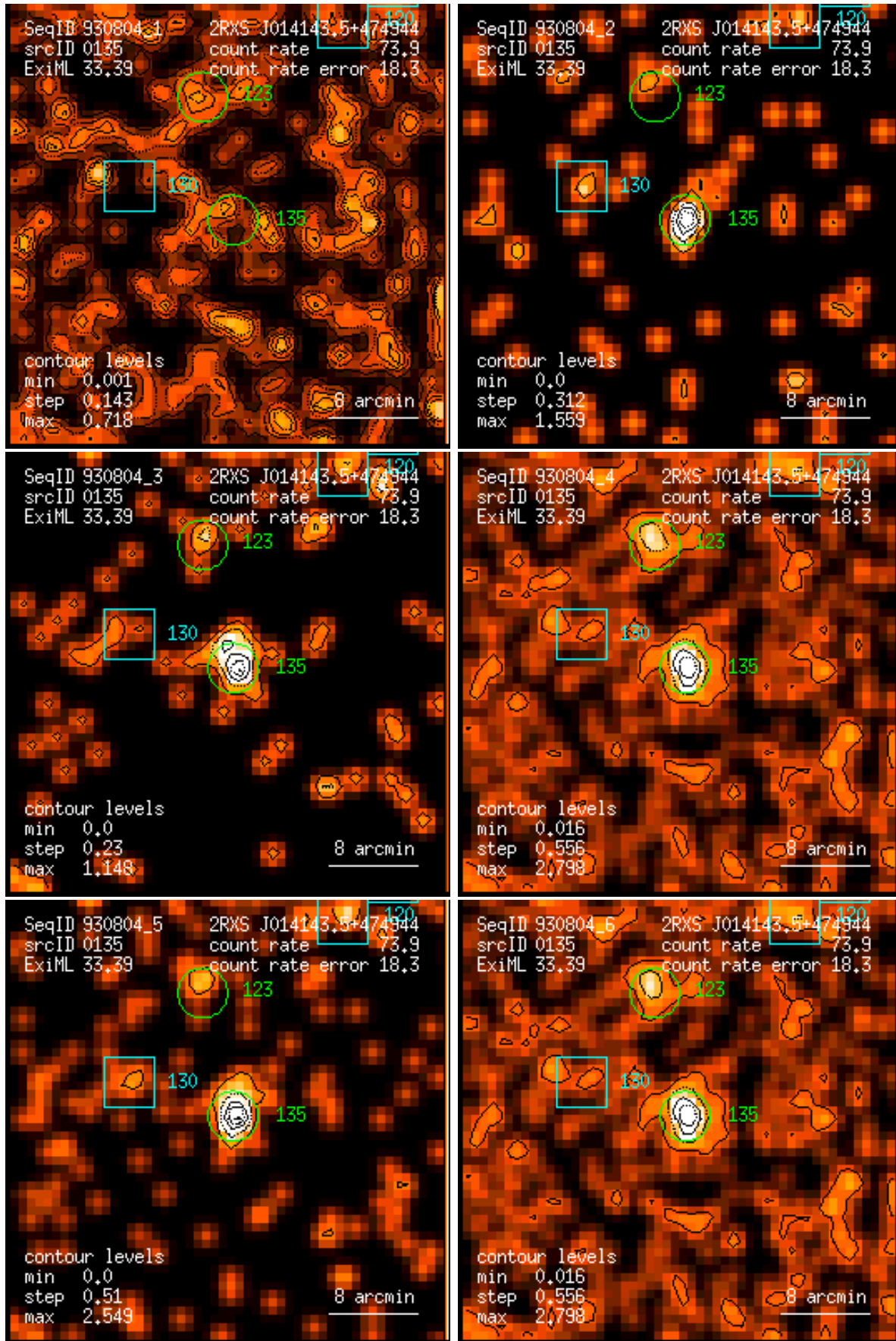
Figure 135: RASS 930804: detection 0135: band rate images, Gaussian filter: (1) PSPC channels 11 – 41, (2) 52 – 90, (3) 91 – 201, (4) 11 – 235, (5) 52 – 201, (6) 11 – 201. Broad band rates in counts/ks. Band rate contour levels in counts/ks/arcmin 2 .
