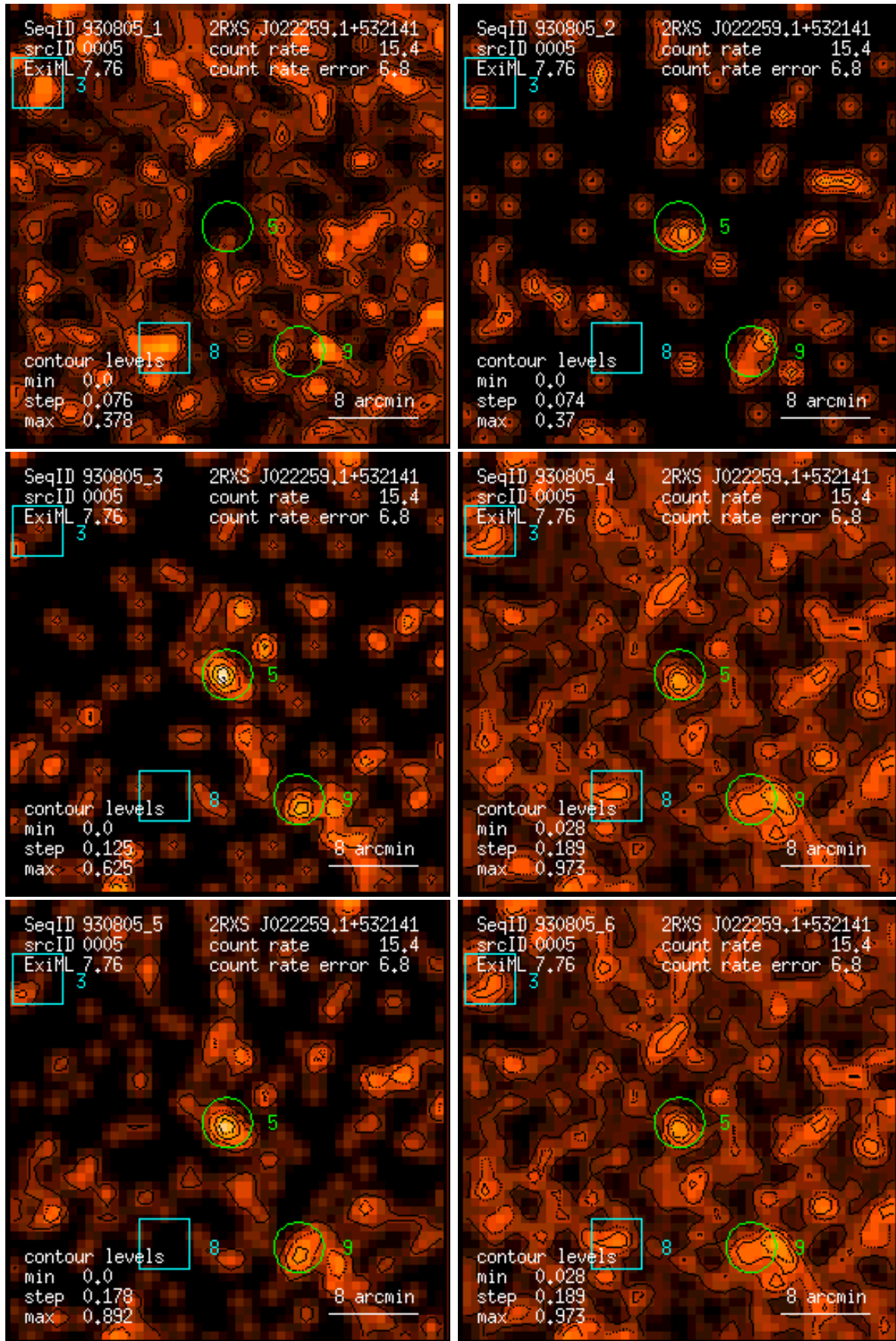
Figure 5: RASS 930805: detection 0005: band rate images, Gaussian filter: (1) PSPC channels 11 – 41, (2) 52 – 90, (3) 91 – 201, (4) 11 – 235, (5) 52 – 201, (6) 11 – 201. Broad band rates in counts/ks. Band rate contour levels in counts/ks/arcmin 2 .
