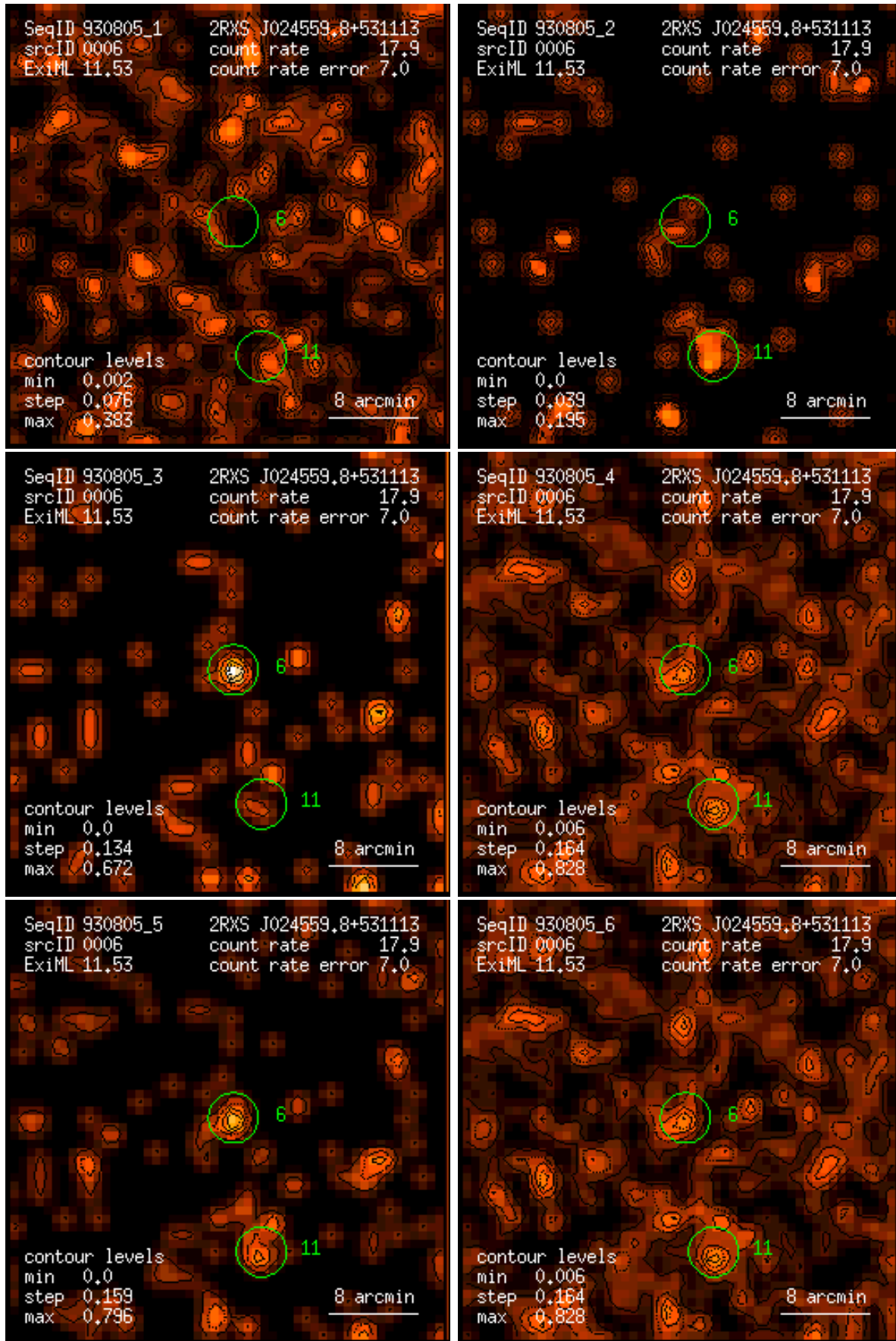
Figure 6: RASS 930805: detection 0006: band rate images, Gaussian filter: (1) PSPC channels 11 – 41, (2) 52 – 90, (3) 91 – 201, (4) 11 – 235, (5) 52 – 201, (6) 11 – 201. Broad band rates in counts/ks. Band rate contour levels in counts/ks/arcmin 2 .
