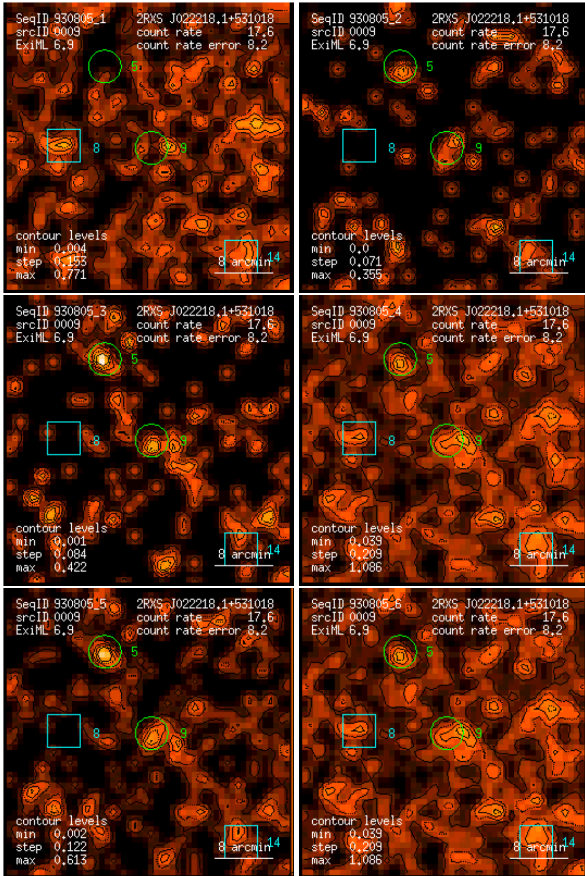
Figure 9: RASS 930805: detection 0009: band rate images, Gaussian filter: (1) PSPC channels 11 – 41, (2) 52 – 90, (3) 91 – 201, (4) 11 – 235, (5) 52 – 201, (6) 11 – 201. Broad band rates in counts/ks. Band rate contour levels in counts/ks/arcmin 2 .
