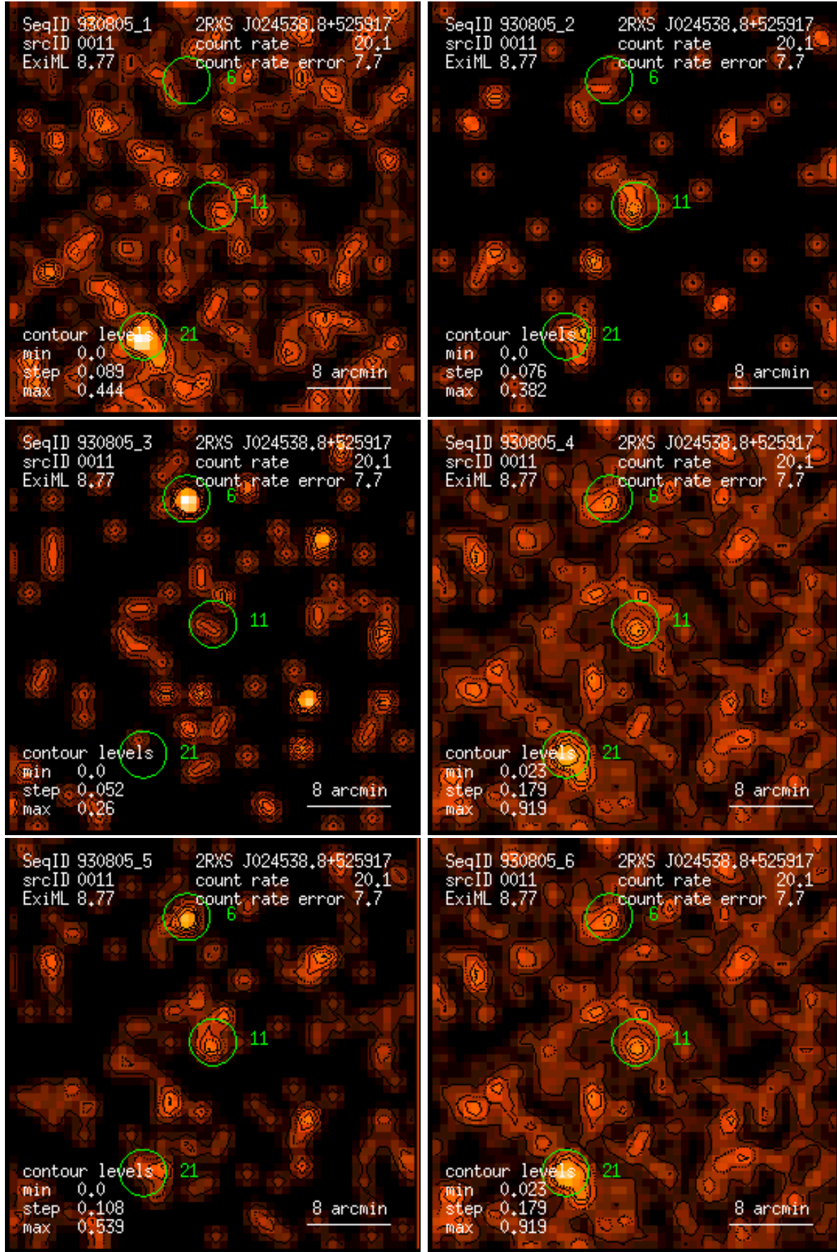
Figure 11: RASS 930805: detection 0011: band rate images, Gaussian filter: (1) PSPC channels 11 – 41, (2) 52 – 90, (3) 91 – 201, (4) 11 – 235, (5) 52 – 201, (6) 11 – 201. Broad band rates in counts/ks. Band rate contour levels in counts/ks/arcmin 2 .
