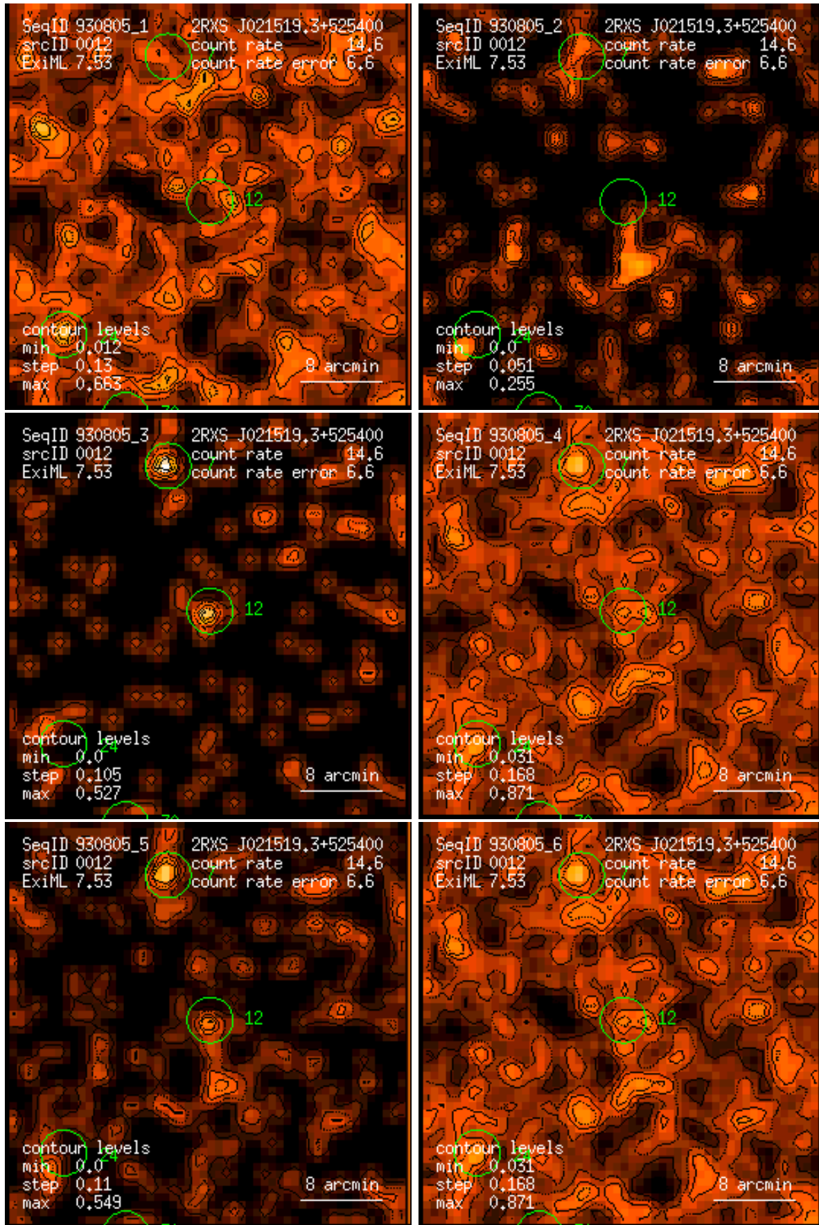
Figure 12: RASS 930805: detection 0012: band rate images, Gaussian filter: (1) PSPC channels 11 – 41, (2) 52 – 90, (3) 91 – 201, (4) 11 – 235, (5) 52 – 201, (6) 11 – 201. Broad band rates in counts/ks. Band rate contour levels in counts/ks/arcmin 2 .
