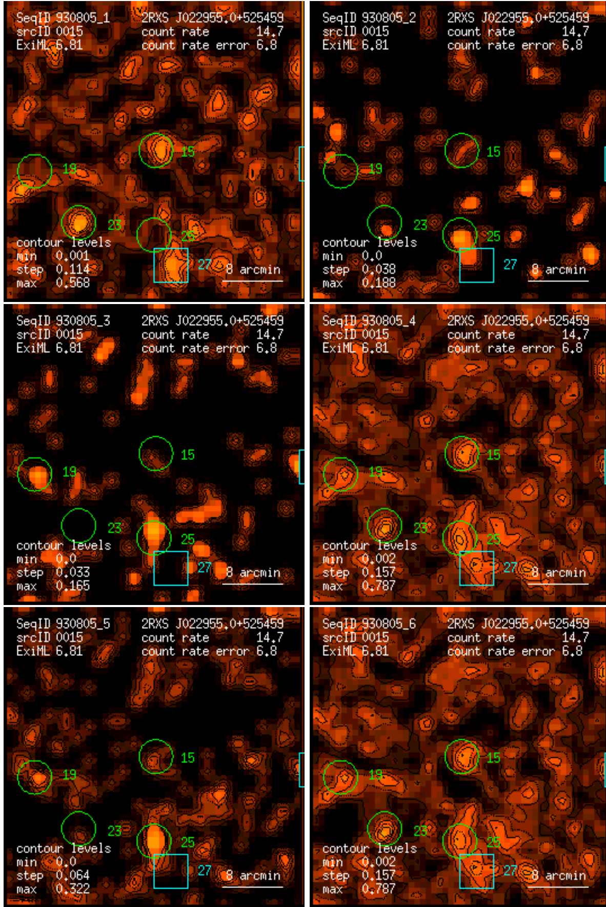
Figure 15: RASS 930805: detection 0015: band rate images, Gaussian filter: (1) PSPC channels 11 – 41, (2) 52 – 90, (3) 91 – 201, (4) 11 – 235, (5) 52 – 201, (6) 11 – 201. Broad band rates in counts/ks. Band rate contour levels in counts/ks/arcmin 2 .
