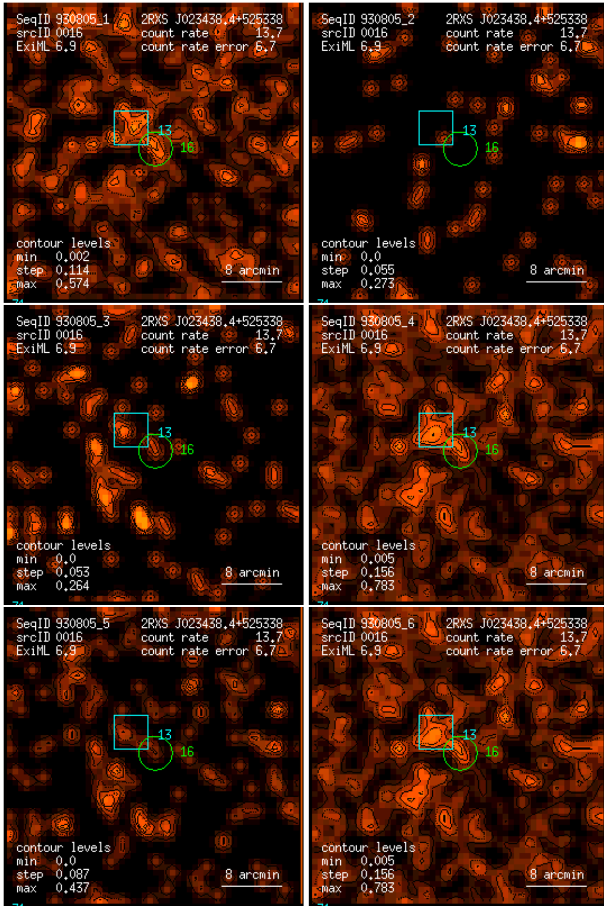
Figure 16: RASS 930805: detection 0016: band rate images, Gaussian filter: (1) PSPC channels 11 – 41, (2) 52 – 90, (3) 91 – 201, (4) 11 – 235, (5) 52 – 201, (6) 11 – 201. Broad band rates in counts/ks. Band rate contour levels in counts/ks/arcmin 2 .
