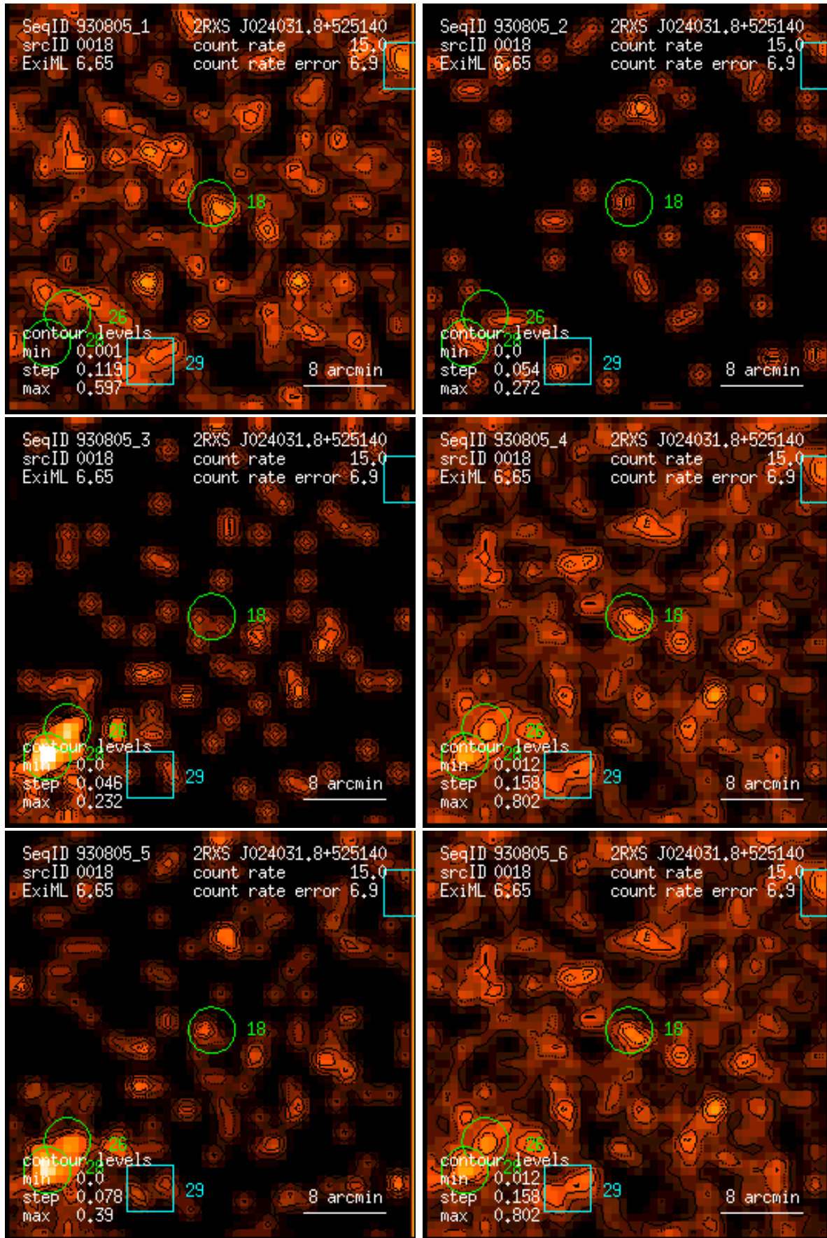
Figure 18: RASS 930805: detection 0018: band rate images, Gaussian filter: (1) PSPC channels 11 – 41, (2) 52 – 90, (3) 91 – 201, (4) 11 – 235, (5) 52 – 201, (6) 11 – 201. Broad band rates in counts/ks. Band rate contour levels in counts/ks/arcmin 2 .
