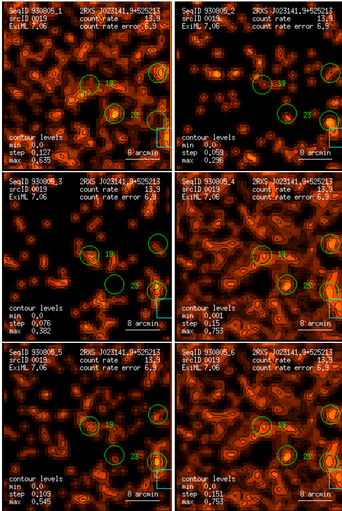
Figure 19: RASS 930805: detection 0019: band rate images, Gaussian filter: (1) PSPC channels 11 – 41, (2) 52 – 90, (3) 91 – 201, (4) 11 – 235, (5) 52 – 201, (6) 11 – 201. Broad band rates in counts/ks. Band rate contour levels in counts/ks/arcmin 2 .
