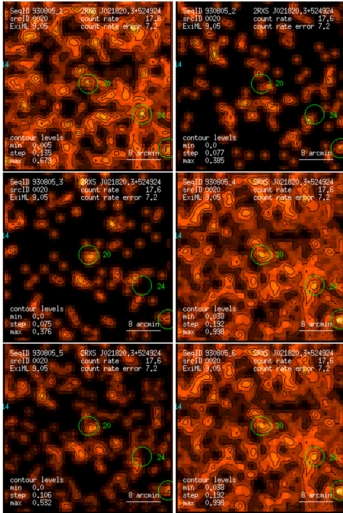
Figure 20: RASS 930805: detection 0020: band rate images, Gaussian filter: (1) PSPC channels 11 – 41, (2) 52 – 90, (3) 91 – 201, (4) 11 – 235, (5) 52 – 201, (6) 11 – 201. Broad band rates in counts/ks. Band rate contour levels in counts/ks/arcmin 2 .
