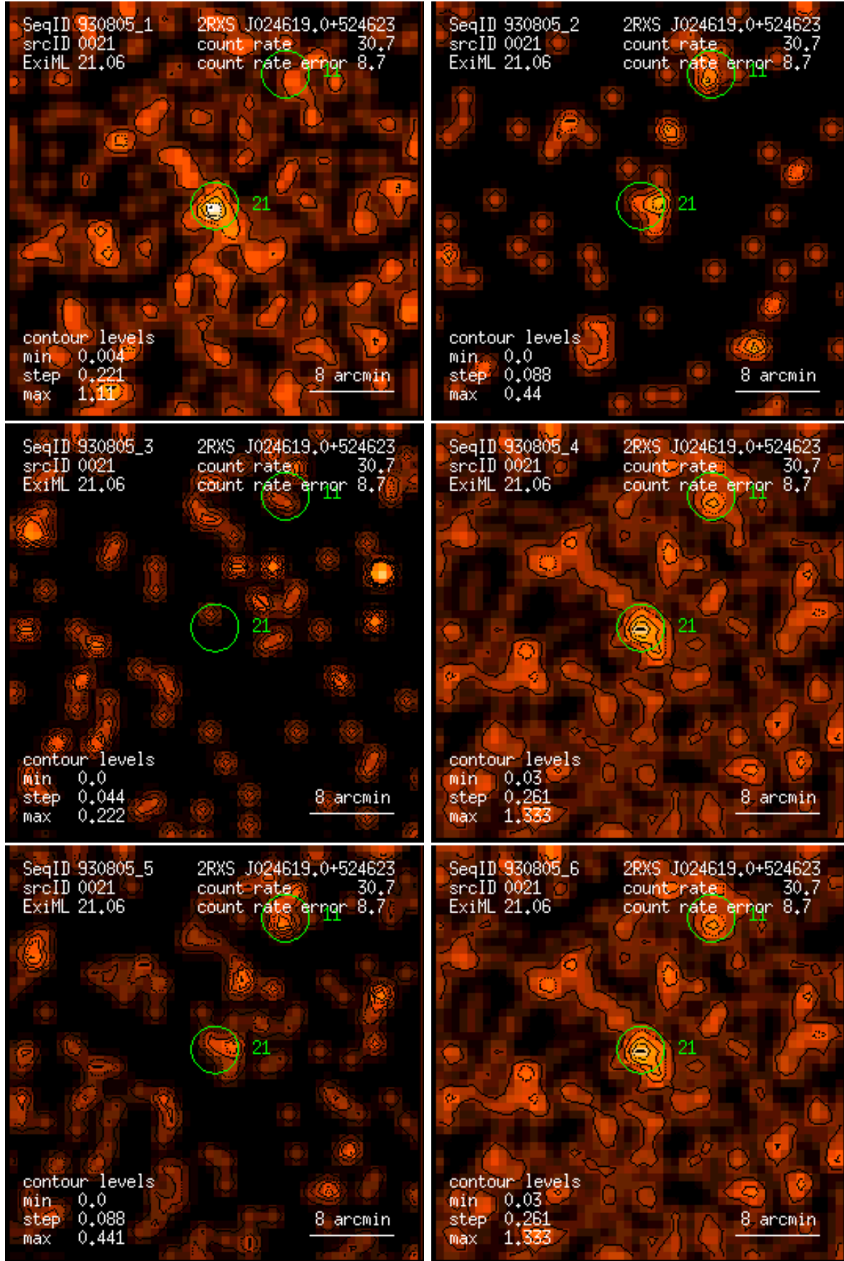
Figure 21: RASS 930805: detection 0021: band rate images, Gaussian filter: (1) PSPC channels 11 – 41, (2) 52 – 90, (3) 91 – 201, (4) 11 – 235, (5) 52 – 201, (6) 11 – 201. Broad band rates in counts/ks. Band rate contour levels in counts/ks/arcmin 2 .
