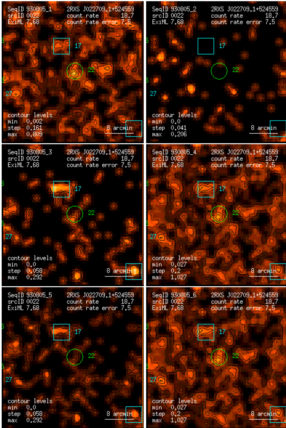
Figure 22: RASS 930805: detection 0022: band rate images, Gaussian filter: (1) PSPC channels 11 – 41, (2) 52 – 90, (3) 91 – 201, (4) 11 – 235, (5) 52 – 201, (6) 11 – 201. Broad band rates in counts/ks. Band rate contour levels in counts/ks/arcmin 2 .
